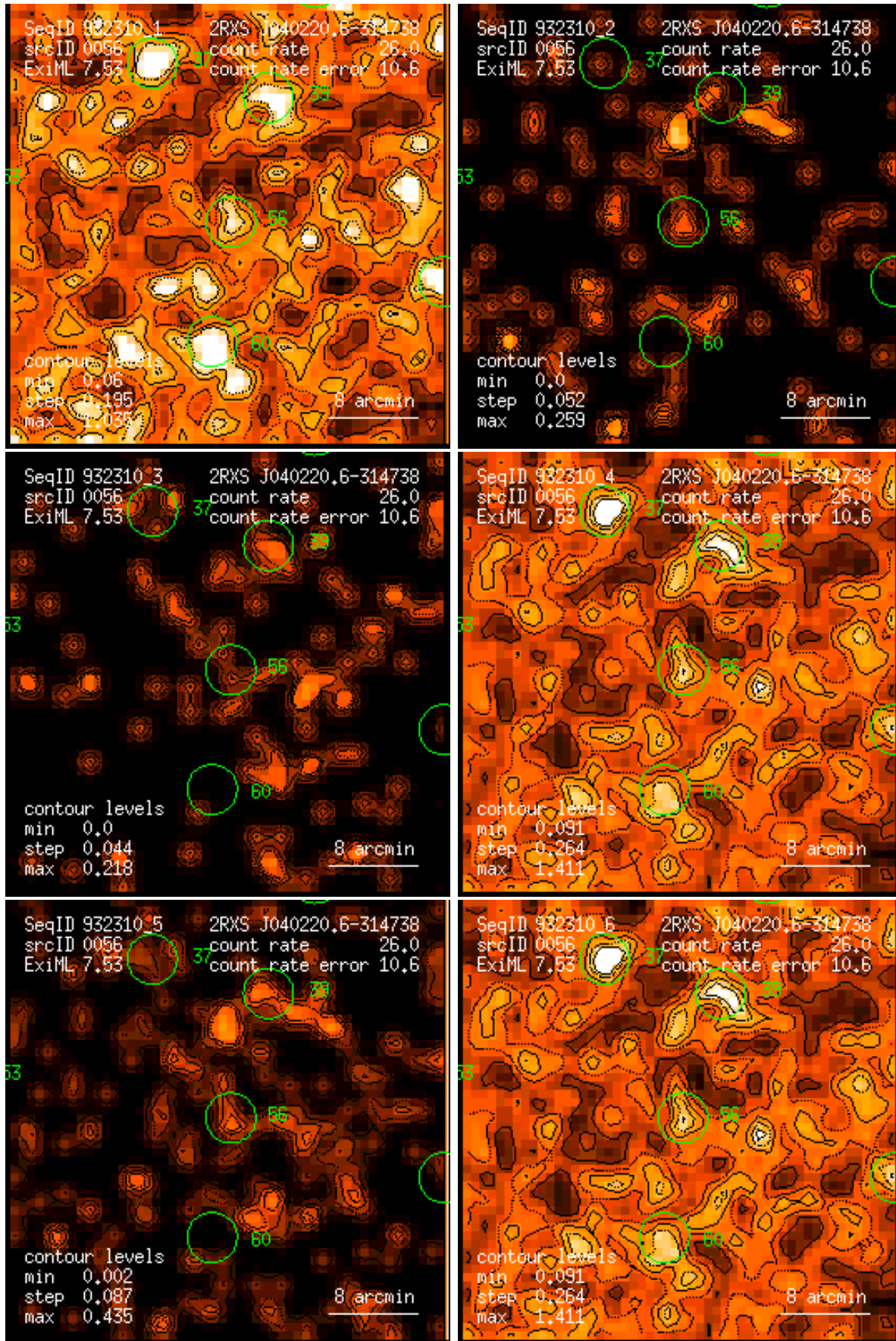
Figure 56: RASS 932310: detection 0056: band rate images, Gaussian filter: (1) PSPC channels 11 – 41, (2) 52 – 90, (3) 91 – 201, (4) 11 – 235, (5) 52 – 201, (6) 11 – 201. Broad band rates in counts/ks. Band rate contour levels in counts/ks/arcmin 2 .
