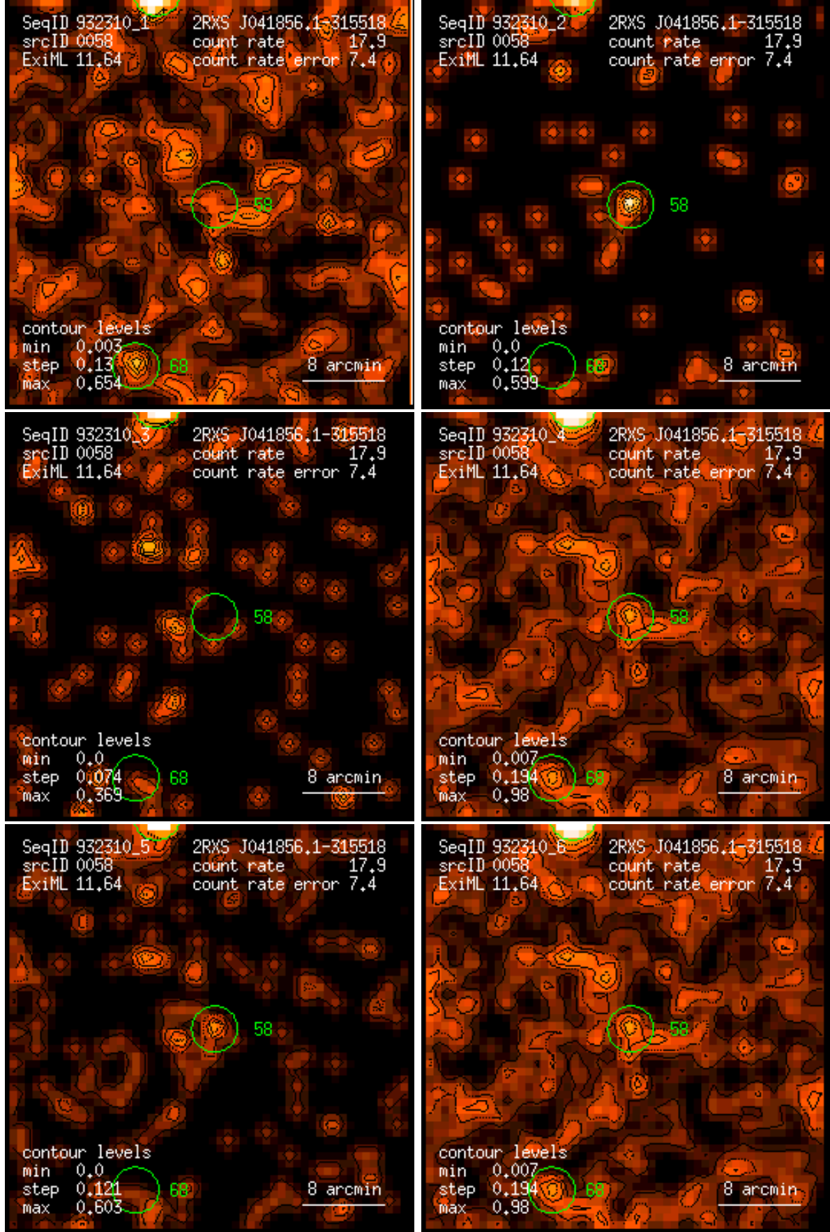
Figure 58: RASS 932310: detection 0058: band rate images, Gaussian filter: (1) PSPC channels 11 – 41, (2) 52 – 90, (3) 91 – 201, (4) 11 – 235, (5) 52 – 201, (6) 11 – 201. Broad band rates in counts/ks. Band rate contour levels in counts/ks/arcmin 2 .
