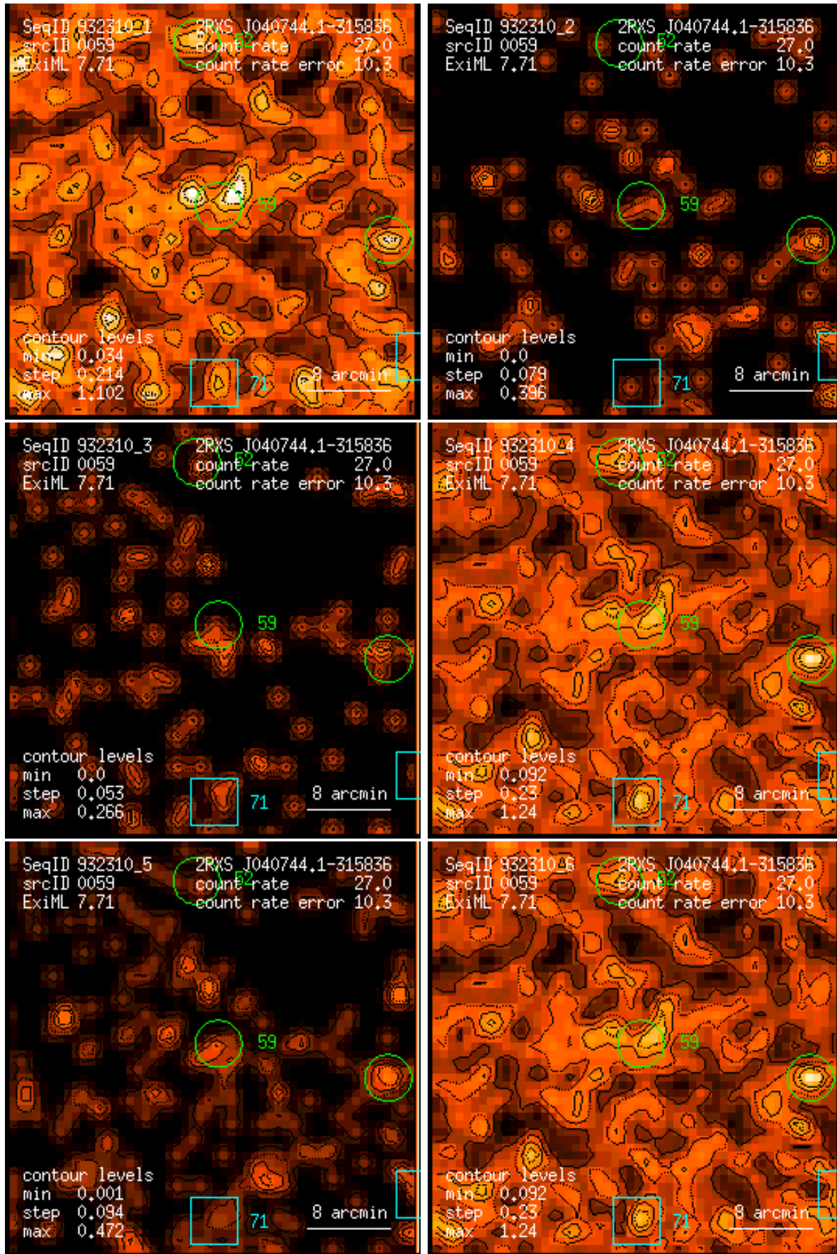
Figure 59: RASS 932310: detection 0059: band rate images, Gaussian filter: (1) PSPC channels 11 – 41, (2) 52 – 90, (3) 91 – 201, (4) 11 – 235, (5) 52 – 201, (6) 11 – 201. Broad band rates in counts/ks. Band rate contour levels in counts/ks/arcmin 2 .
