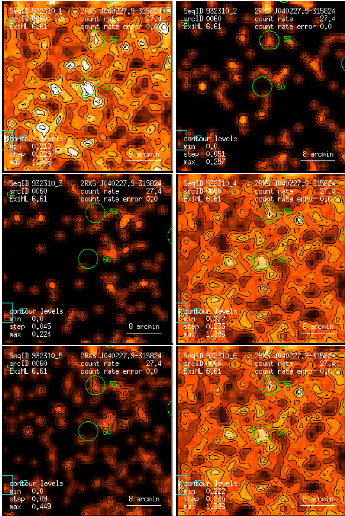
Figure 60: RASS 932310: detection 0060: band rate images, Gaussian filter: (1) PSPC channels 11 – 41, (2) 52 – 90, (3) 91 – 201, (4) 11 – 235, (5) 52 – 201, (6) 11 – 201. Broad band rates in counts/ks. Band rate contour levels in counts/ks/arcmin 2 .
