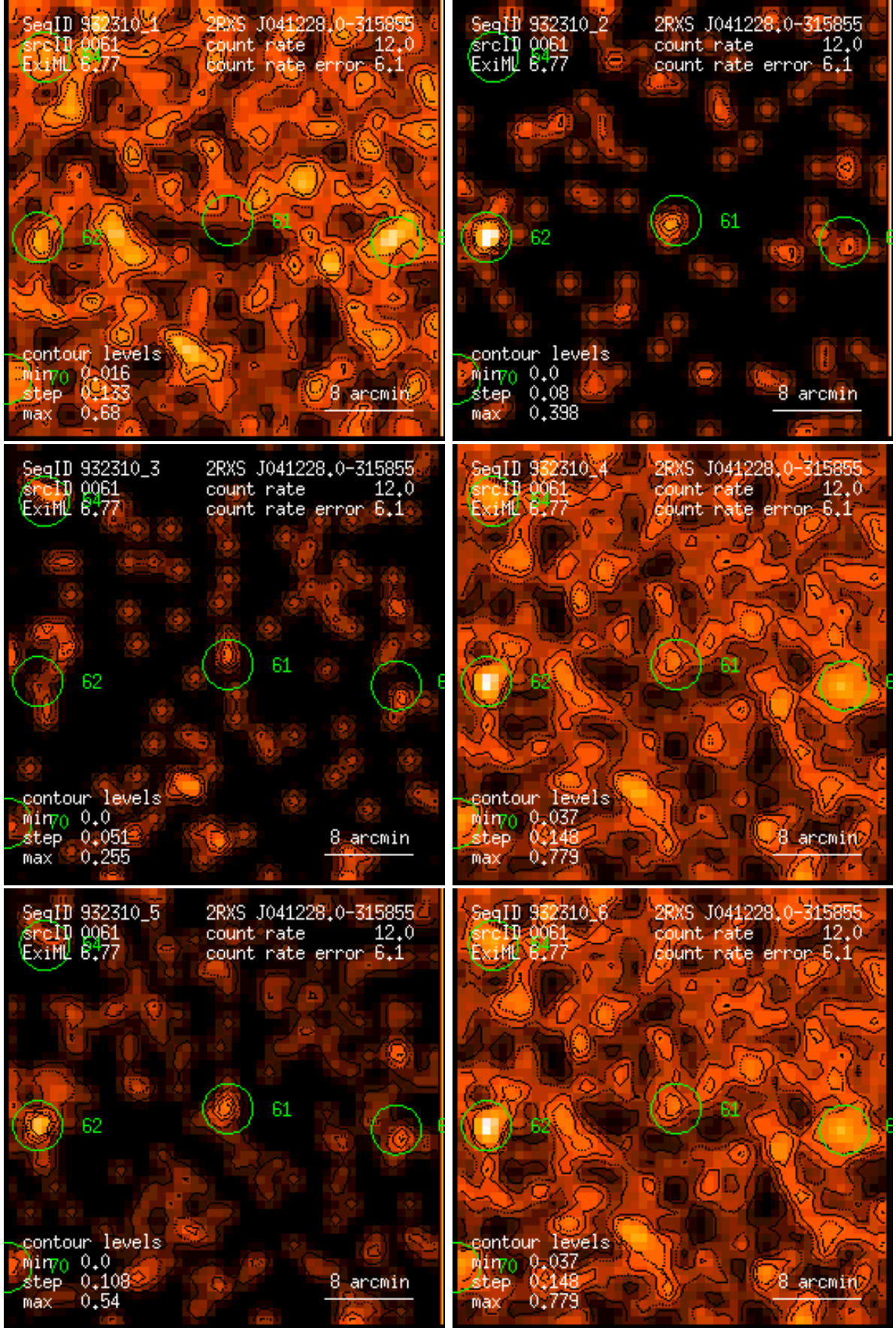
Figure 61: RASS 932310: detection 0061: band rate images, Gaussian filter: (1) PSPC channels 11 – 41, (2) 52 – 90, (3) 91 – 201, (4) 11 – 235, (5) 52 – 201, (6) 11 – 201. Broad band rates in counts/ks. Band rate contour levels in counts/ks/arcmin 2 .
