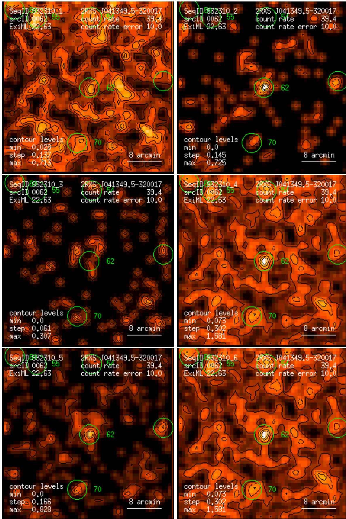
Figure 62: RASS 932310: detection 0062: band rate images, Gaussian filter: (1) PSPC channels 11 – 41, (2) 52 – 90, (3) 91 – 201, (4) 11 – 235, (5) 52 – 201, (6) 11 – 201. Broad band rates in counts/ks. Band rate contour levels in counts/ks/arcmin 2 .
