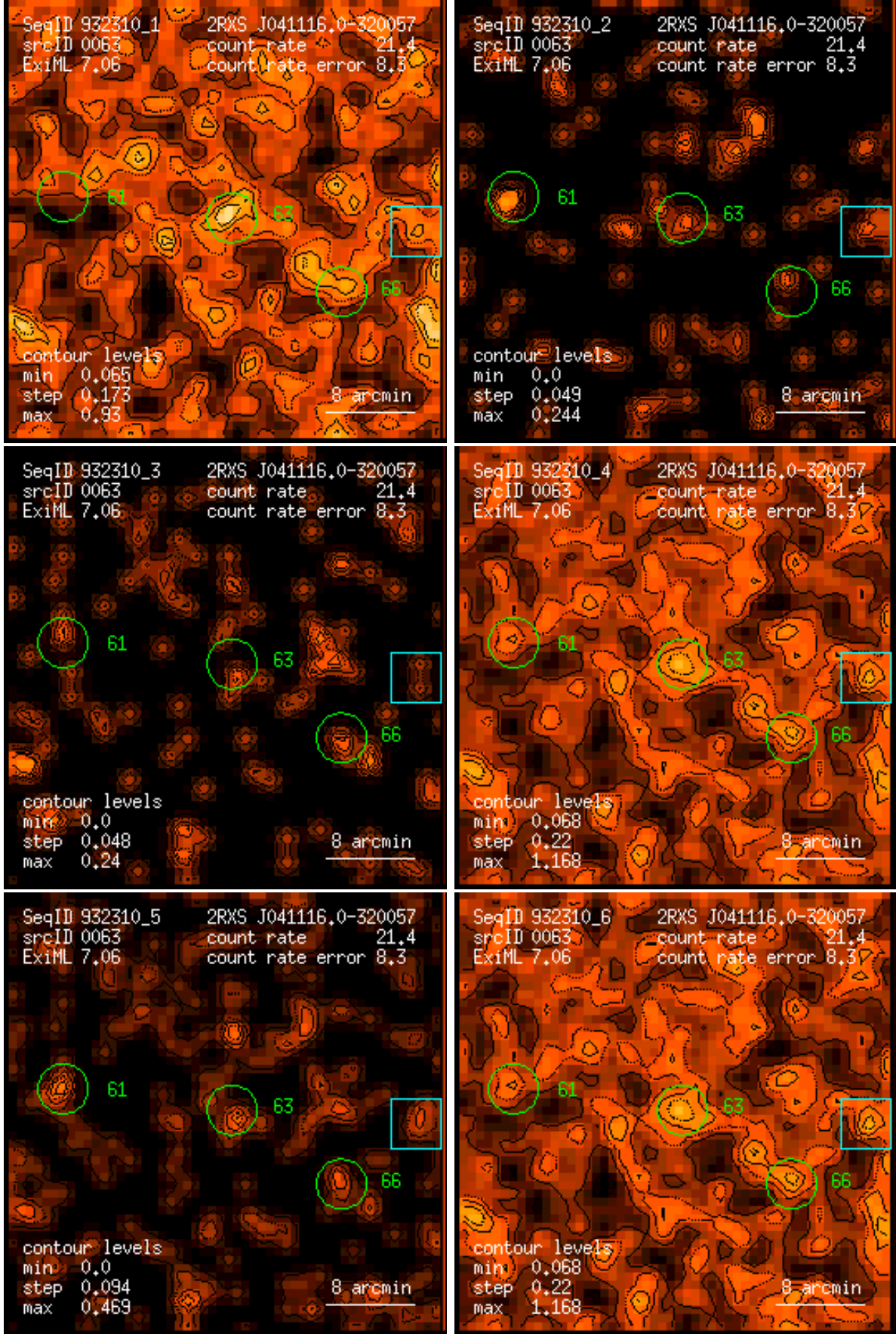
Figure 63: RASS 932310: detection 0063: band rate images, Gaussian filter: (1) PSPC channels 11 – 41, (2) 52 – 90, (3) 91 – 201, (4) 11 – 235, (5) 52 – 201, (6) 11 – 201. Broad band rates in counts/ks. Band rate contour levels in counts/ks/arcmin 2 .
