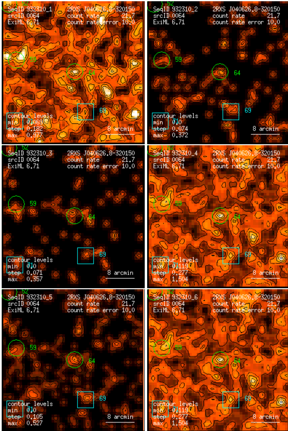
Figure 64: RASS 932310: detection 0064: band rate images, Gaussian filter: (1) PSPC channels 11 – 41, (2) 52 – 90, (3) 91 – 201, (4) 11 – 235, (5) 52 – 201, (6) 11 – 201. Broad band rates in counts/ks. Band rate contour levels in counts/ks/arcmin 2 .
