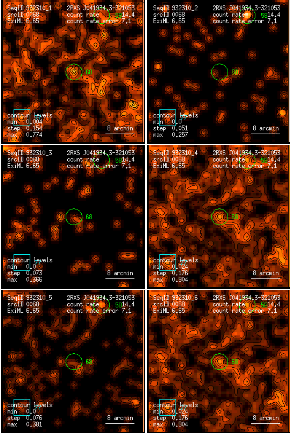
Figure 68: RASS 932310: detection 0068: band rate images, Gaussian filter: (1) PSPC channels 11 – 41, (2) 52 – 90, (3) 91 – 201, (4) 11 – 235, (5) 52 – 201, (6) 11 – 201. Broad band rates in counts/ks. Band rate contour levels in counts/ks/arcmin 2 .
