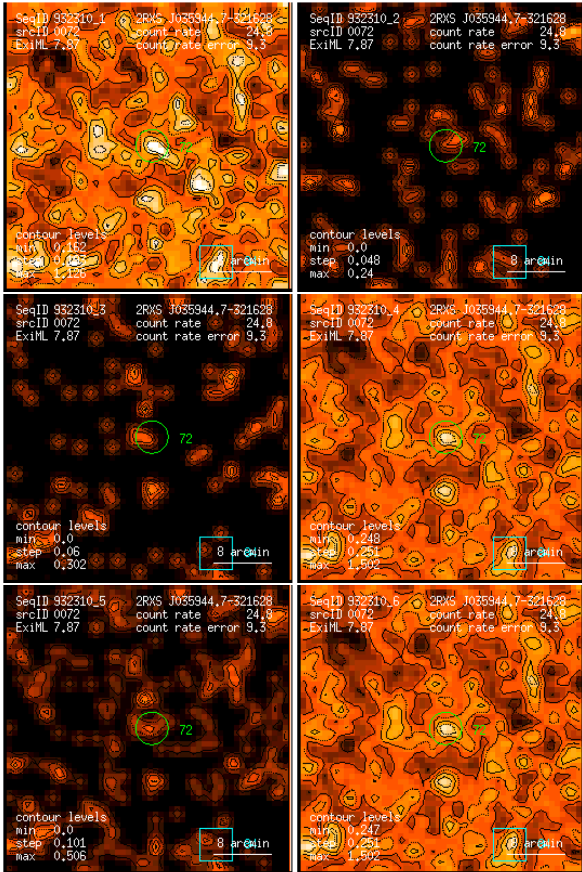
Figure 72: RASS 932310: detection 0072: band rate images, Gaussian filter: (1) PSPC channels 11 – 41, (2) 52 – 90, (3) 91 – 201, (4) 11 – 235, (5) 52 – 201, (6) 11 – 201. Broad band rates in counts/ks. Band rate contour levels in counts/ks/arcmin 2 .
