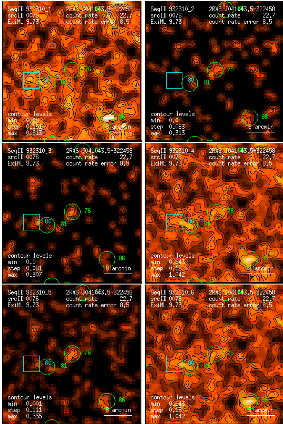
Figure 76: RASS 932310: detection 0076: band rate images, Gaussian filter: (1) PSPC channels 11 – 41, (2) 52 – 90, (3) 91 – 201, (4) 11 – 235, (5) 52 – 201, (6) 11 – 201. Broad band rates in counts/ks. Band rate contour levels in counts/ks/arcmin 2 .
