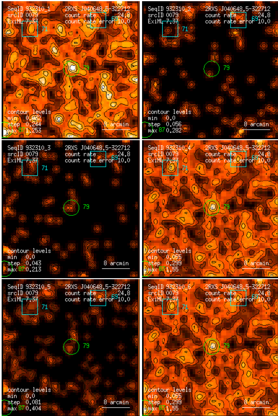
Figure 79: RASS 932310: detection 0079: band rate images, Gaussian filter: (1) PSPC channels 11 – 41, (2) 52 – 90, (3) 91 – 201, (4) 11 – 235, (5) 52 – 201, (6) 11 – 201. Broad band rates in counts/ks. Band rate contour levels in counts/ks/arcmin 2 .
