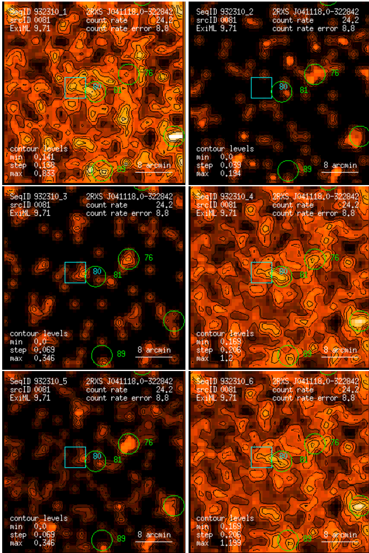
Figure 81: RASS 932310: detection 0081: band rate images, Gaussian filter: (1) PSPC channels 11 – 41, (2) 52 – 90, (3) 91 – 201, (4) 11 – 235, (5) 52 – 201, (6) 11 – 201. Broad band rates in counts/ks. Band rate contour levels in counts/ks/arcmin 2 .
