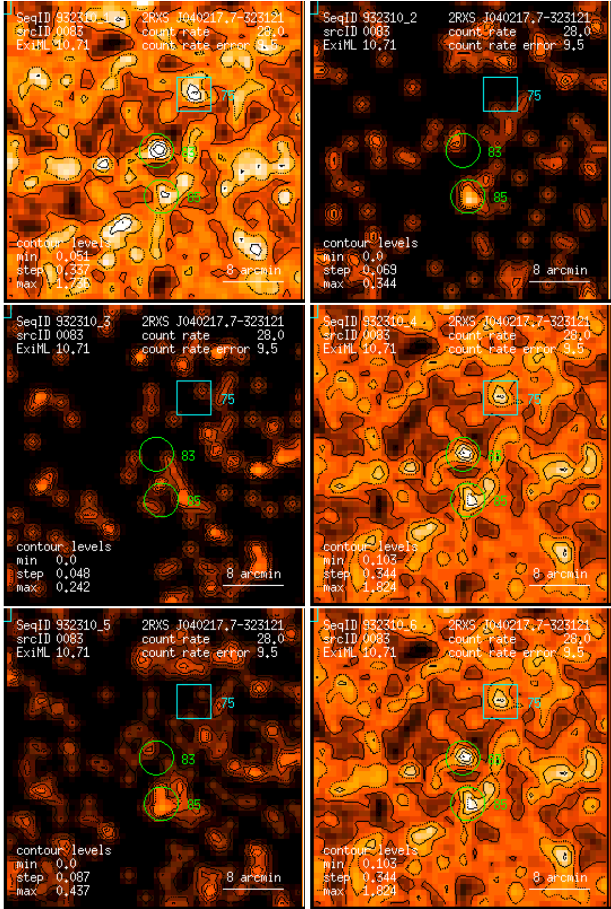
Figure 83: RASS 932310: detection 0083: band rate images, Gaussian filter: (1) PSPC channels 11 – 41, (2) 52 – 90, (3) 91 – 201, (4) 11 – 235, (5) 52 – 201, (6) 11 – 201. Broad band rates in counts/ks. Band rate contour levels in counts/ks/arcmin 2 .
