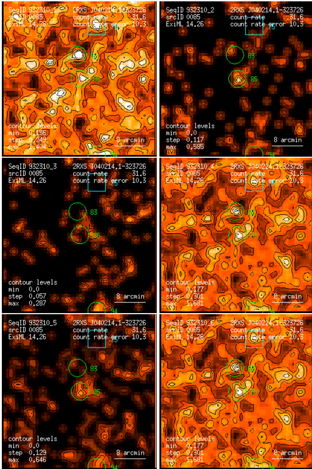
Figure 85: RASS 932310: detection 0085: band rate images, Gaussian filter: (1) PSPC channels 11 – 41, (2) 52 – 90, (3) 91 – 201, (4) 11 – 235, (5) 52 – 201, (6) 11 – 201. Broad band rates in counts/ks. Band rate contour levels in counts/ks/arcmin 2 .
