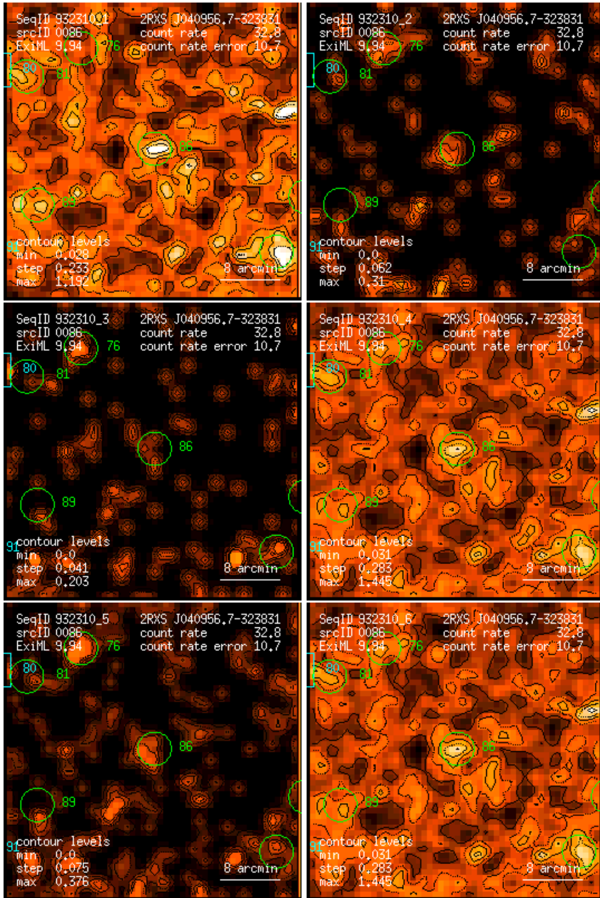
Figure 86: RASS 932310: detection 0086: band rate images, Gaussian filter: (1) PSPC channels 11 – 41, (2) 52 – 90, (3) 91 – 201, (4) 11 – 235, (5) 52 – 201, (6) 11 – 201. Broad band rates in counts/ks. Band rate contour levels in counts/ks/arcmin 2 .
