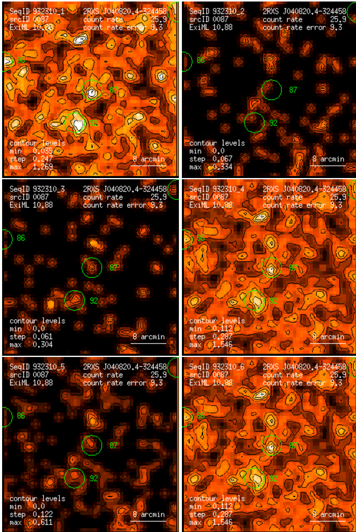
Figure 87: RASS 932310: detection 0087: band rate images, Gaussian filter: (1) PSPC channels 11 – 41, (2) 52 – 90, (3) 91 – 201, (4) 11 – 235, (5) 52 – 201, (6) 11 – 201. Broad band rates in counts/ks. Band rate contour levels in counts/ks/arcmin 2 .
