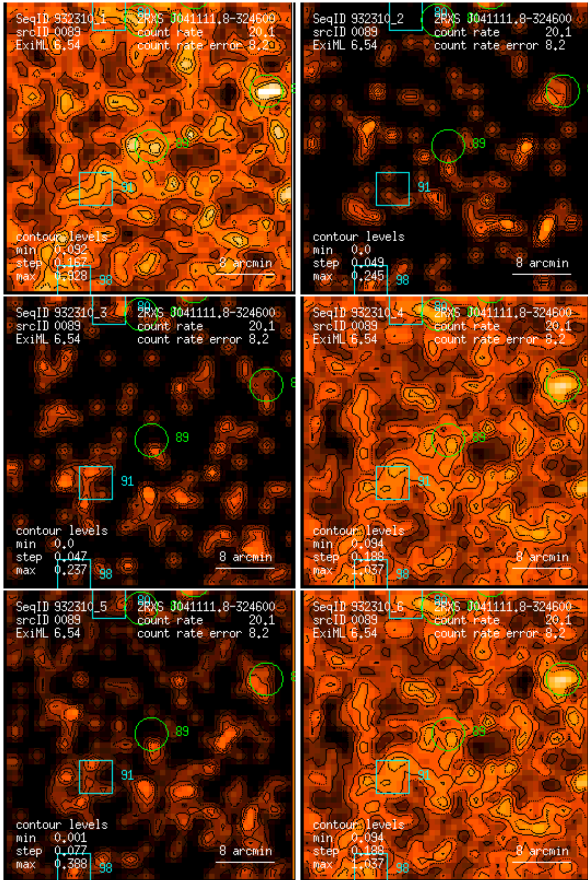
Figure 89: RASS 932310: detection 0089: band rate images, Gaussian filter: (1) PSPC channels 11 – 41, (2) 52 – 90, (3) 91 – 201, (4) 11 – 235, (5) 52 – 201, (6) 11 – 201. Broad band rates in counts/ks. Band rate contour levels in counts/ks/arcmin 2 .
