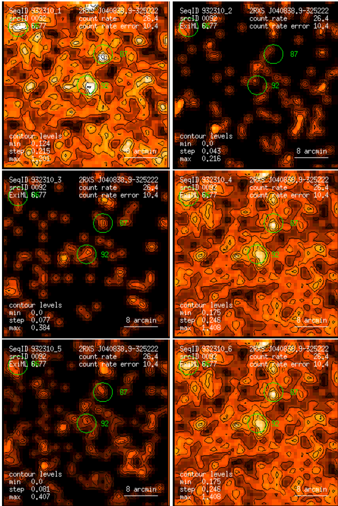
Figure 92: RASS 932310: detection 0092: band rate images, Gaussian filter: (1) PSPC channels 11 – 41, (2) 52 – 90, (3) 91 – 201, (4) 11 – 235, (5) 52 – 201, (6) 11 – 201. Broad band rates in counts/ks. Band rate contour levels in counts/ks/arcmin 2 .
