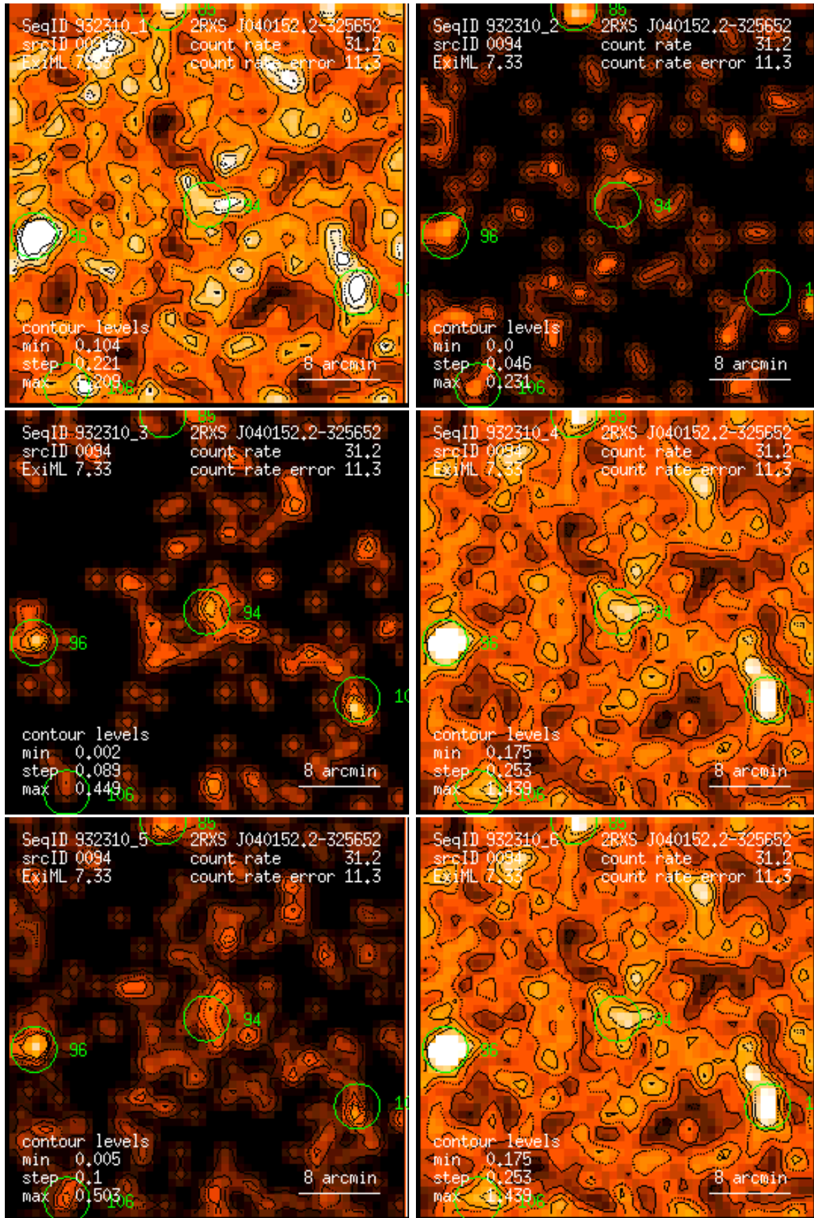
Figure 94: RASS 932310: detection 0094: band rate images, Gaussian filter: (1) PSPC channels 11 – 41, (2) 52 – 90, (3) 91 – 201, (4) 11 – 235, (5) 52 – 201, (6) 11 – 201. Broad band rates in counts/ks. Band rate contour levels in counts/ks/arcmin 2 .
