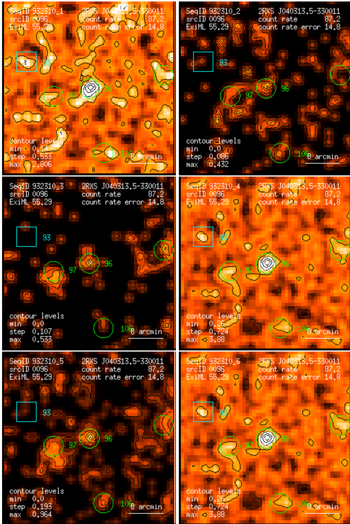
Figure 96: RASS 932310: detection 0096: band rate images, Gaussian filter: (1) PSPC channels 11 – 41, (2) 52 – 90, (3) 91 – 201, (4) 11 – 235, (5) 52 – 201, (6) 11 – 201. Broad band rates in counts/ks. Band rate contour levels in counts/ks/arcmin 2 .
