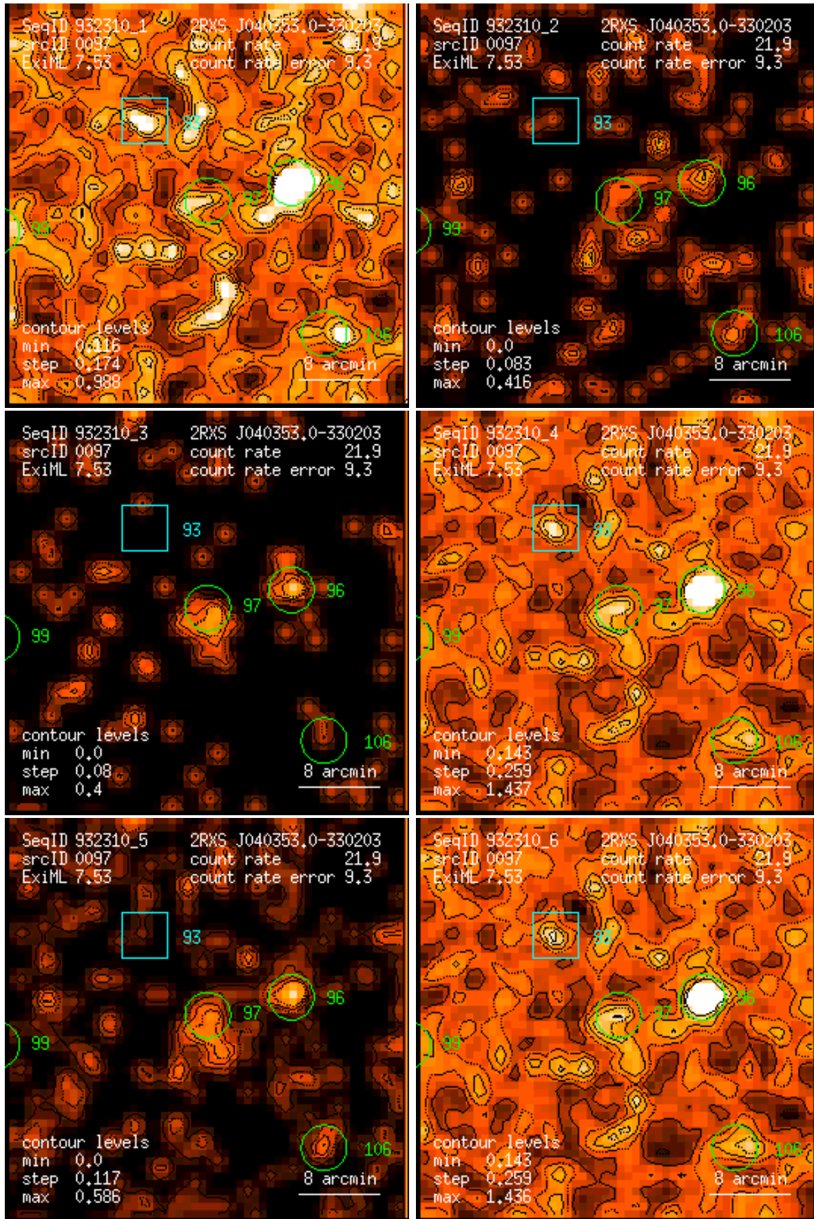
Figure 97: RASS 932310: detection 0097: band rate images, Gaussian filter: (1) PSPC channels 11 – 41, (2) 52 – 90, (3) 91 – 201, (4) 11 – 235, (5) 52 – 201, (6) 11 – 201. Broad band rates in counts/ks. Band rate contour levels in counts/ks/arcmin 2 .
