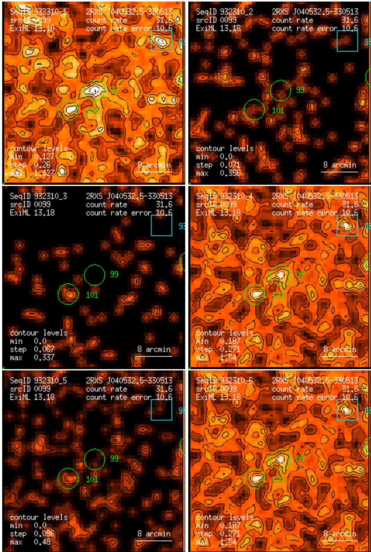
Figure 99: RASS 932310: detection 0099: band rate images, Gaussian filter: (1) PSPC channels 11 – 41, (2) 52 – 90, (3) 91 – 201, (4) 11 – 235, (5) 52 – 201, (6) 11 – 201. Broad band rates in counts/ks. Band rate contour levels in counts/ks/arcmin 2 .
