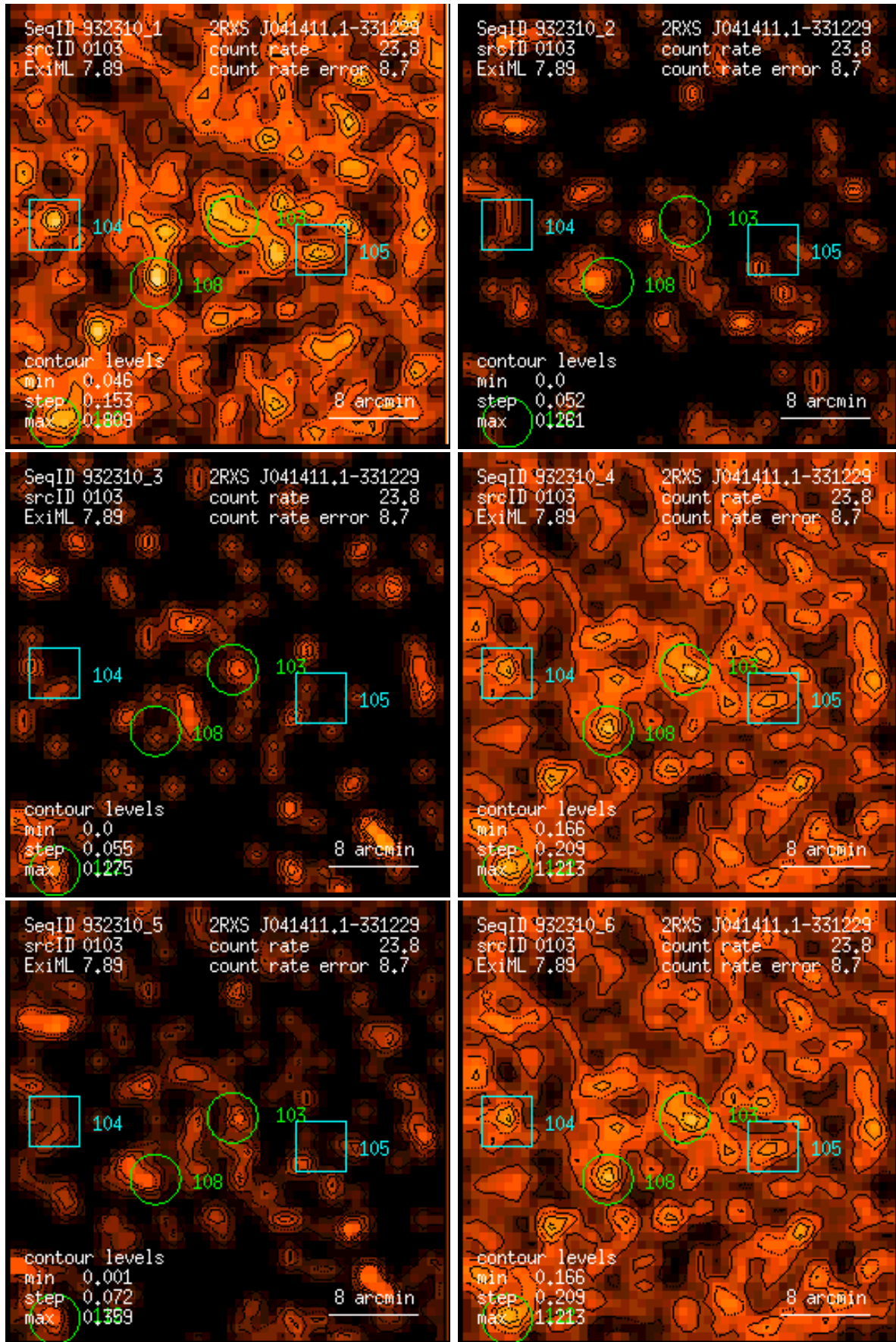
Figure 103: RASS 932310: detection 0103: band rate images, Gaussian filter: (1) PSPC channels 11 – 41, (2) 52 – 90, (3) 91 – 201, (4) 11 – 235, (5) 52 – 201, (6) 11 – 201. Broad band rates in counts/ks. Band rate contour levels in counts/ks/arcmin 2 .
