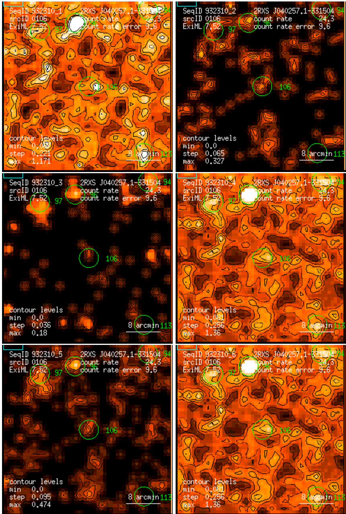
Figure 106: RASS 932310: detection 0106: band rate images, Gaussian filter: (1) PSPC channels 11 – 41, (2) 52 – 90, (3) 91 – 201, (4) 11 – 235, (5) 52 – 201, (6) 11 – 201. Broad band rates in counts/ks. Band rate contour levels in counts/ks/arcmin 2 .
