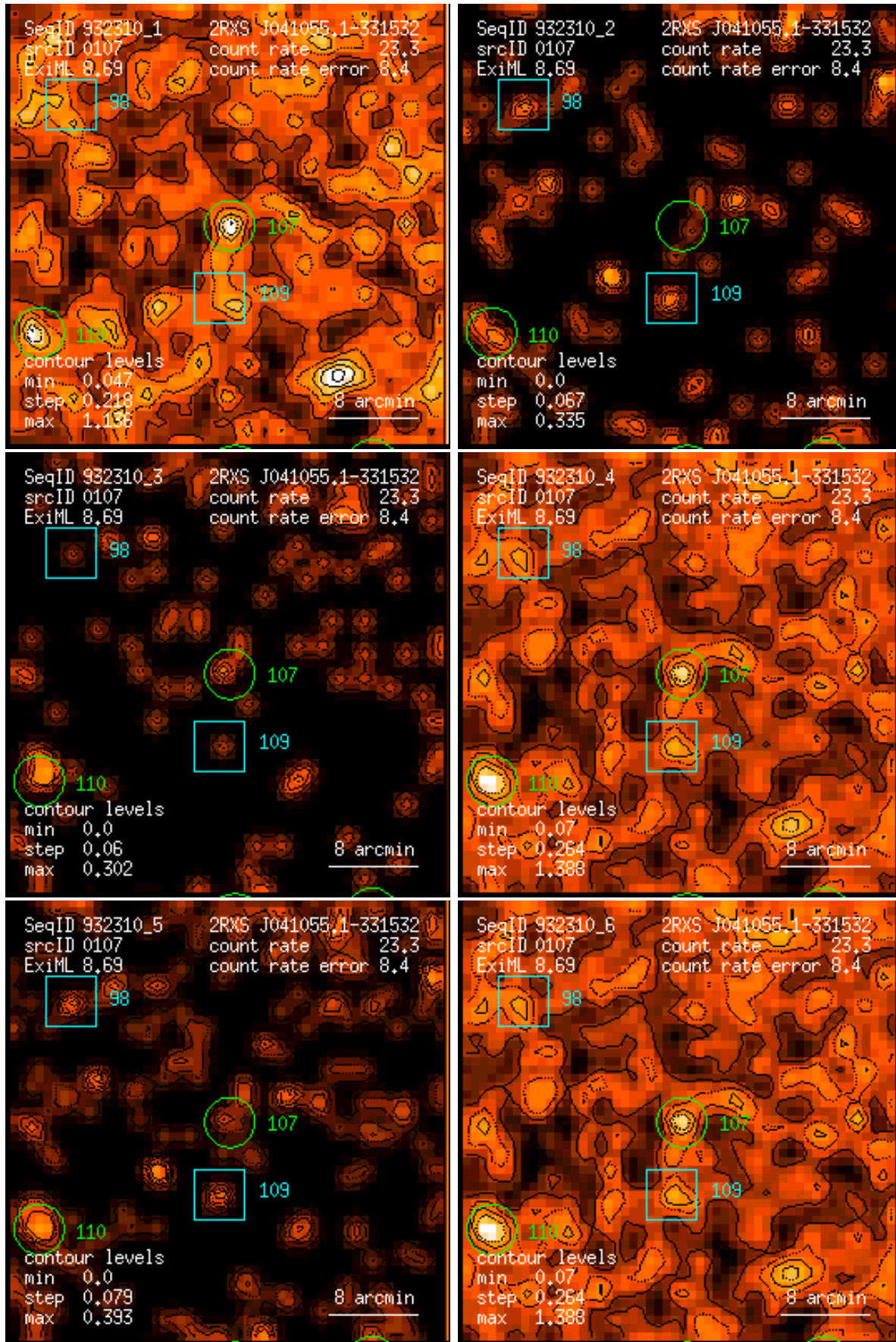
Figure 107: RASS 932310: detection 0107: band rate images, Gaussian filter: (1) PSPC channels 11 – 41, (2) 52 – 90, (3) 91 – 201, (4) 11 – 235, (5) 52 – 201, (6) 11 – 201. Broad band rates in counts/ks. Band rate contour levels in counts/ks/arcmin 2 .
