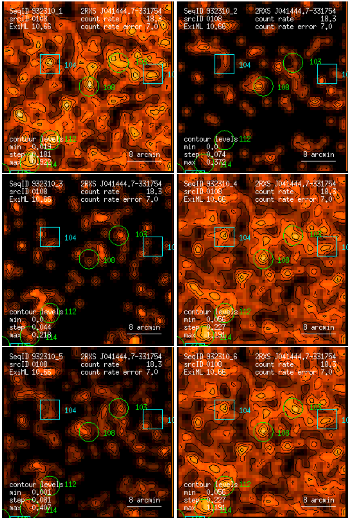
Figure 108: RASS 932310: detection 0108: band rate images, Gaussian filter: (1) PSPC channels 11 – 41, (2) 52 – 90, (3) 91 – 201, (4) 11 – 235, (5) 52 – 201, (6) 11 – 201. Broad band rates in counts/ks. Band rate contour levels in counts/ks/arcmin 2 .
