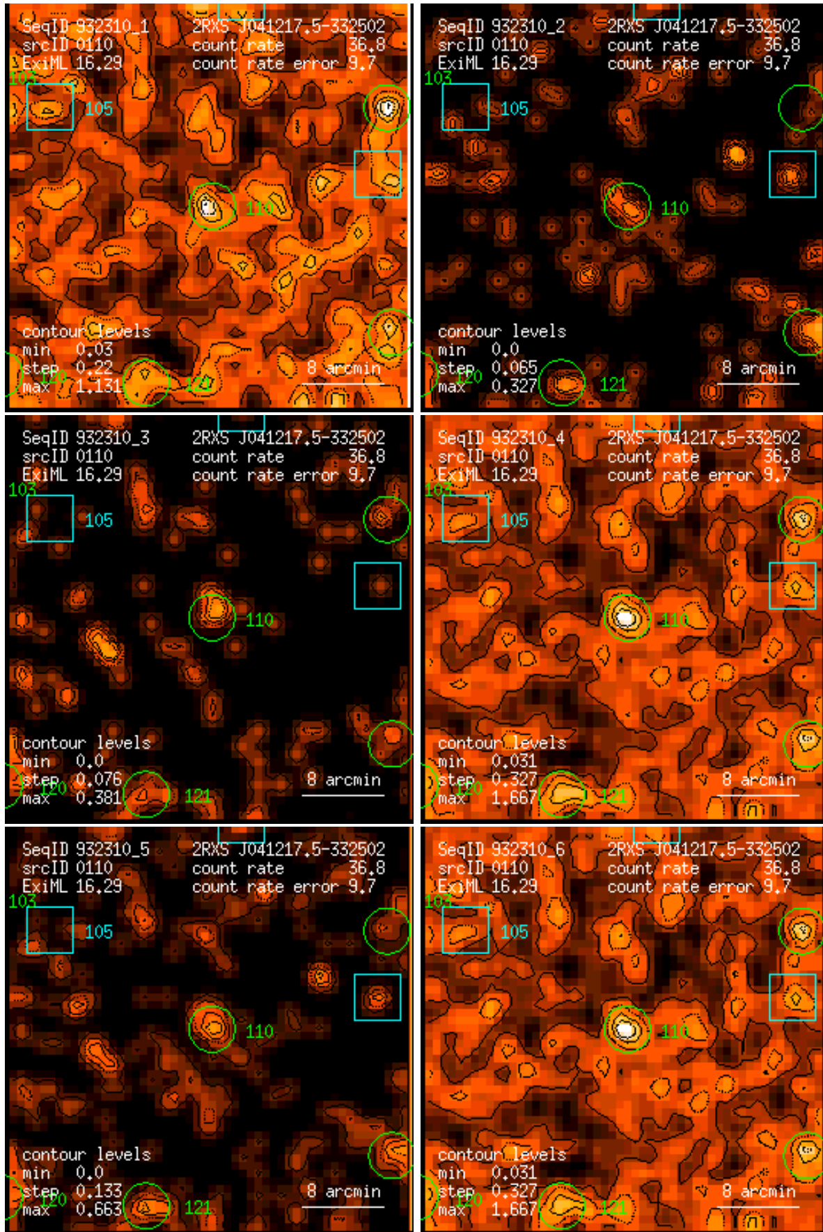
Figure 110: RASS 932310: detection 0110: band rate images, Gaussian filter: (1) PSPC channels 11 – 41, (2) 52 – 90, (3) 91 – 201, (4) 11 – 235, (5) 52 – 201, (6) 11 – 201. Broad band rates in counts/ks. Band rate contour levels in counts/ks/arcmin 2 .
