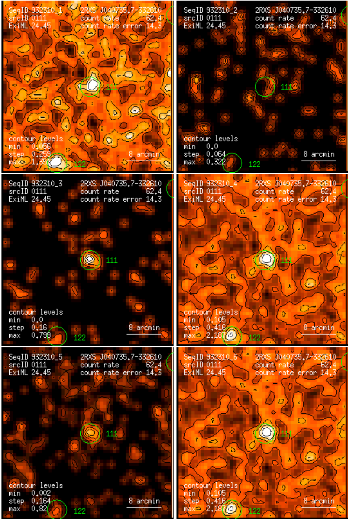
Figure 111: RASS 932310: detection 0111: band rate images, Gaussian filter: (1) PSPC channels 11 – 41, (2) 52 – 90, (3) 91 – 201, (4) 11 – 235, (5) 52 – 201, (6) 11 – 201. Broad band rates in counts/ks. Band rate contour levels in counts/ks/arcmin 2 .
