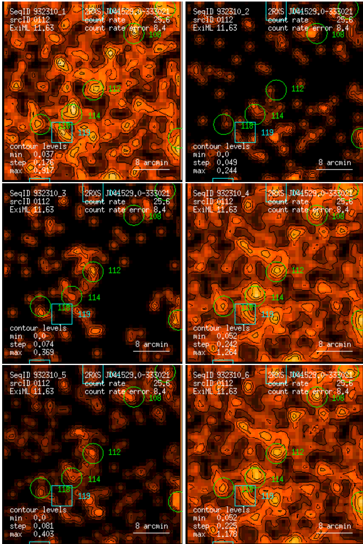
Figure 112: RASS 932310: detection 0112: band rate images, Gaussian filter: (1) PSPC channels 11 – 41, (2) 52 – 90, (3) 91 – 201, (4) 11 – 235, (5) 52 – 201, (6) 11 – 201. Broad band rates in counts/ks. Band rate contour levels in counts/ks/arcmin 2 .
