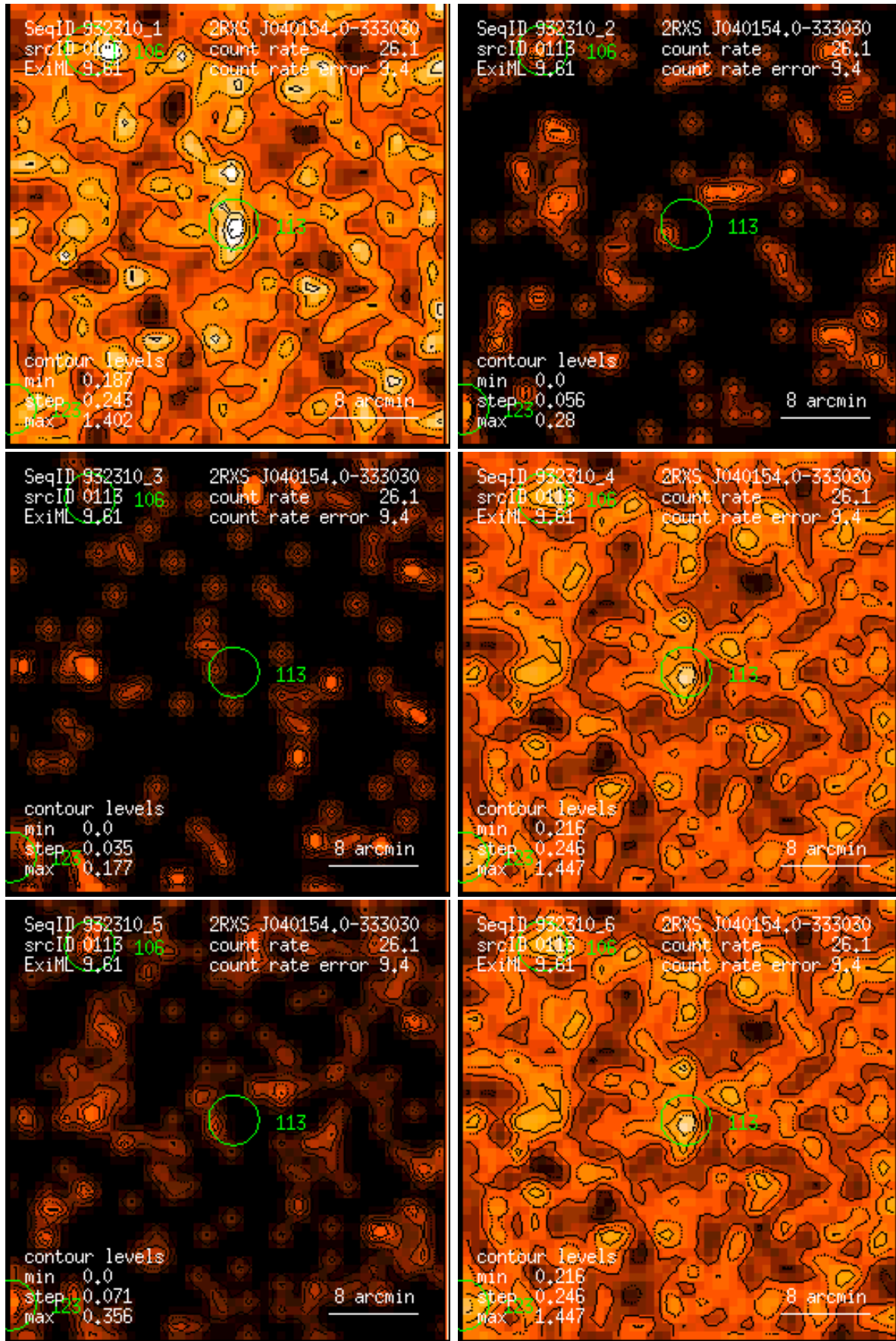
Figure 113: RASS 932310: detection 0113: band rate images, Gaussian filter: (1) PSPC channels 11 – 41, (2) 52 – 90, (3) 91 – 201, (4) 11 – 235, (5) 52 – 201, (6) 11 – 201. Broad band rates in counts/ks. Band rate contour levels in counts/ks/arcmin 2 .
