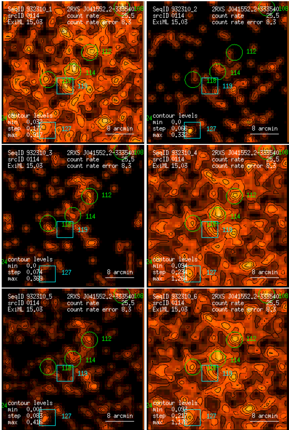
Figure 114: RASS 932310: detection 0114: band rate images, Gaussian filter: (1) PSPC channels 11 – 41, (2) 52 – 90, (3) 91 – 201, (4) 11 – 235, (5) 52 – 201, (6) 11 – 201. Broad band rates in counts/ks. Band rate contour levels in counts/ks/arcmin 2 .
