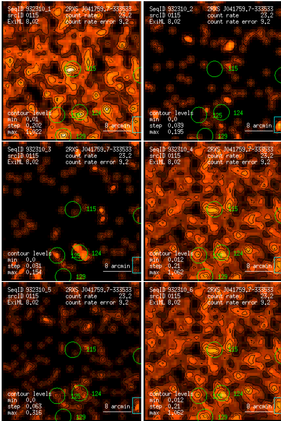
Figure 115: RASS 932310: detection 0115: band rate images, Gaussian filter: (1) PSPC channels 11 – 41, (2) 52 – 90, (3) 91 – 201, (4) 11 – 235, (5) 52 – 201, (6) 11 – 201. Broad band rates in counts/ks. Band rate contour levels in counts/ks/arcmin 2 .
