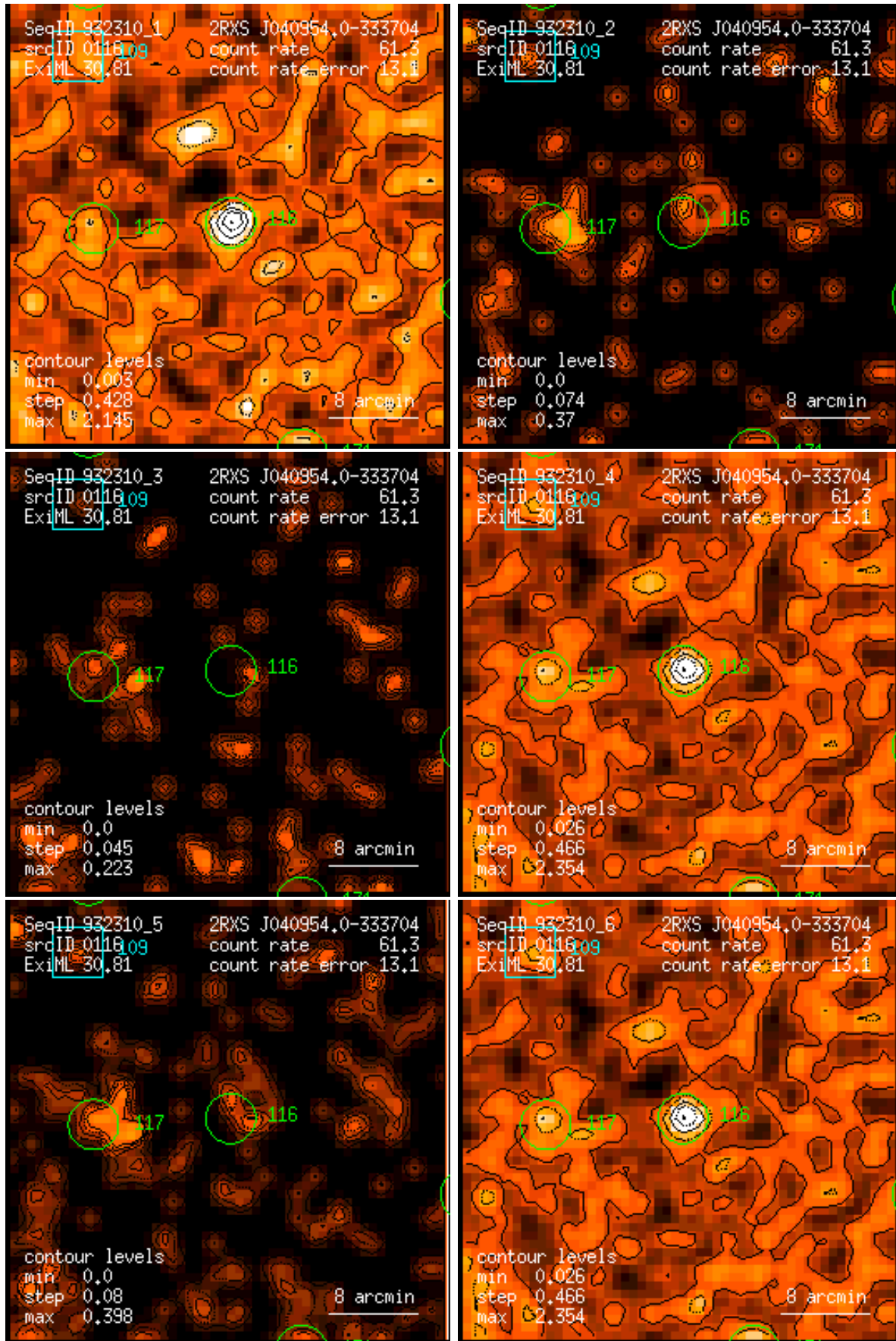
Figure 116: RASS 932310: detection 0116: band rate images, Gaussian filter: (1) PSPC channels 11 – 41, (2) 52 – 90, (3) 91 – 201, (4) 11 – 235, (5) 52 – 201, (6) 11 – 201. Broad band rates in counts/ks. Band rate contour levels in counts/ks/arcmin 2 .
