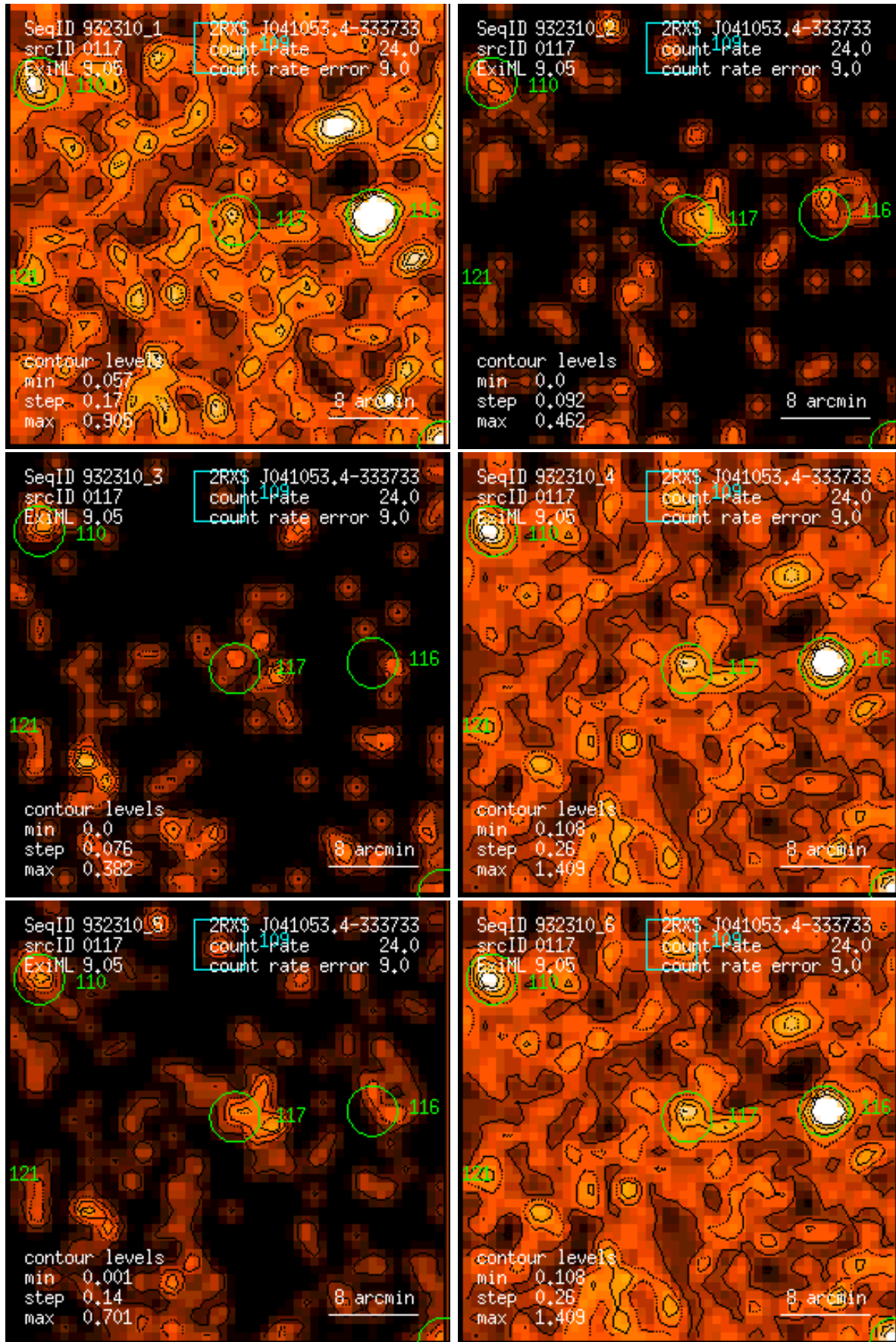
Figure 117: RASS 932310: detection 0117: band rate images, Gaussian filter: (1) PSPC channels 11 – 41, (2) 52 – 90, (3) 91 – 201, (4) 11 – 235, (5) 52 – 201, (6) 11 – 201. Broad band rates in counts/ks. Band rate contour levels in counts/ks/arcmin 2 .
