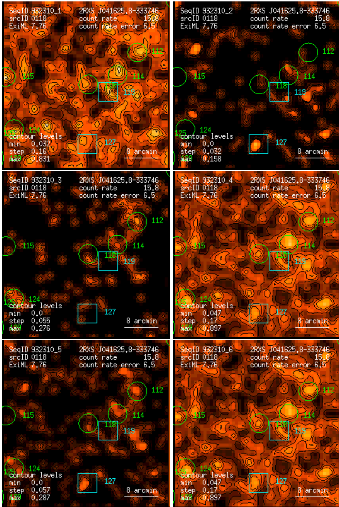
Figure 118: RASS 932310: detection 0118: band rate images, Gaussian filter: (1) PSPC channels 11 – 41, (2) 52 – 90, (3) 91 – 201, (4) 11 – 235, (5) 52 – 201, (6) 11 – 201. Broad band rates in counts/ks. Band rate contour levels in counts/ks/arcmin 2 .
