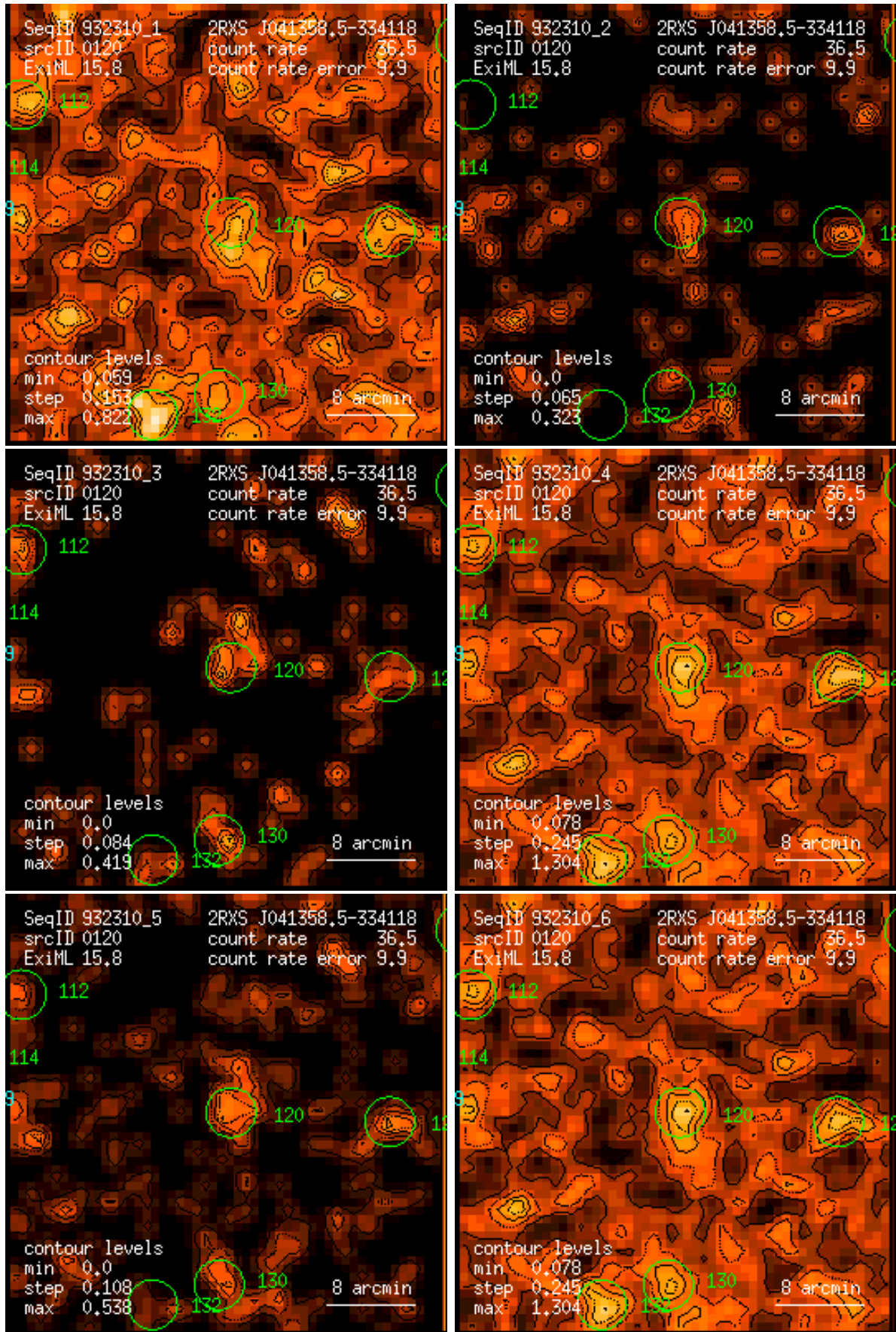
Figure 120: RASS 932310: detection 0120: band rate images, Gaussian filter: (1) PSPC channels 11 – 41, (2) 52 – 90, (3) 91 – 201, (4) 11 – 235, (5) 52 – 201, (6) 11 – 201. Broad band rates in counts/ks. Band rate contour levels in counts/ks/arcmin 2 .
