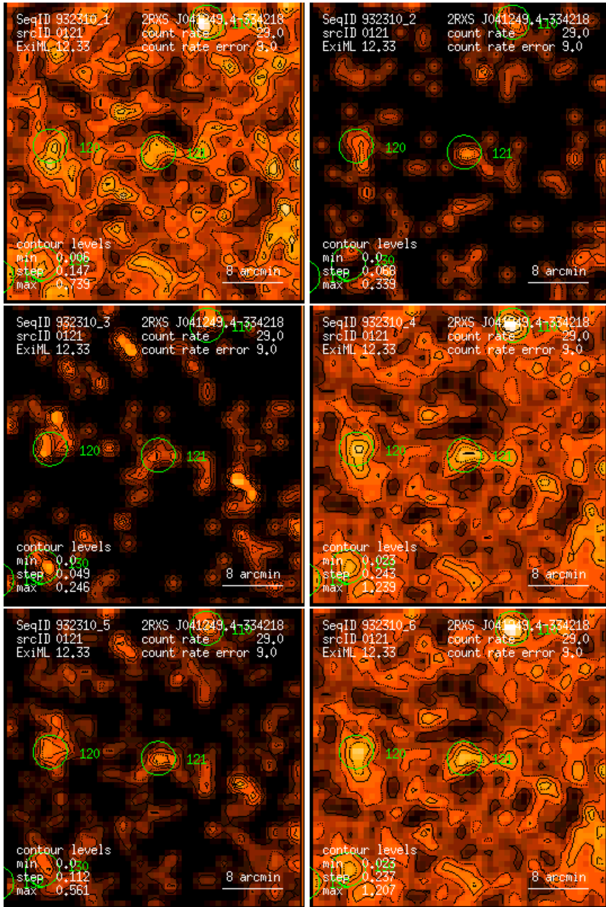
Figure 121: RASS 932310: detection 0121: band rate images, Gaussian filter: (1) PSPC channels 11 – 41, (2) 52 – 90, (3) 91 – 201, (4) 11 – 235, (5) 52 – 201, (6) 11 – 201. Broad band rates in counts/ks. Band rate contour levels in counts/ks/arcmin 2 .
