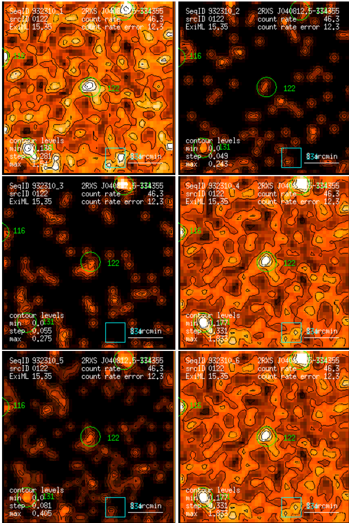
Figure 122: RASS 932310: detection 0122: band rate images, Gaussian filter: (1) PSPC channels 11 – 41, (2) 52 – 90, (3) 91 – 201, (4) 11 – 235, (5) 52 – 201, (6) 11 – 201. Broad band rates in counts/ks. Band rate contour levels in counts/ks/arcmin 2 .
