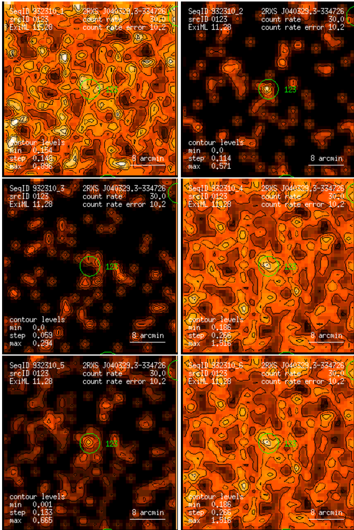
Figure 123: RASS 932310: detection 0123: band rate images, Gaussian filter: (1) PSPC channels 11 – 41, (2) 52 – 90, (3) 91 – 201, (4) 11 – 235, (5) 52 – 201, (6) 11 – 201. Broad band rates in counts/ks. Band rate contour levels in counts/ks/arcmin 2 .
