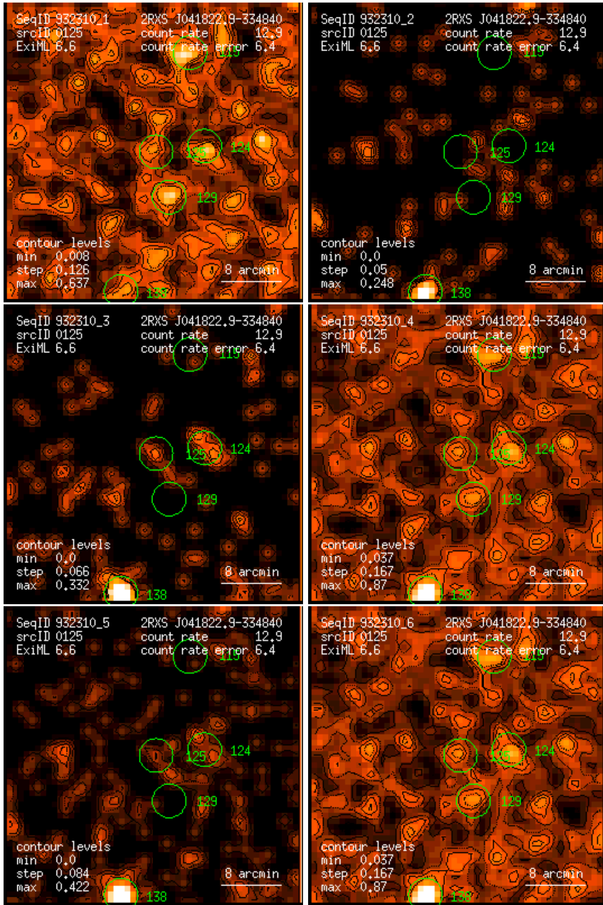
Figure 125: RASS 932310: detection 0125: band rate images, Gaussian filter: (1) PSPC channels 11 – 41, (2) 52 – 90, (3) 91 – 201, (4) 11 – 235, (5) 52 – 201, (6) 11 – 201. Broad band rates in counts/ks. Band rate contour levels in counts/ks/arcmin 2 .
