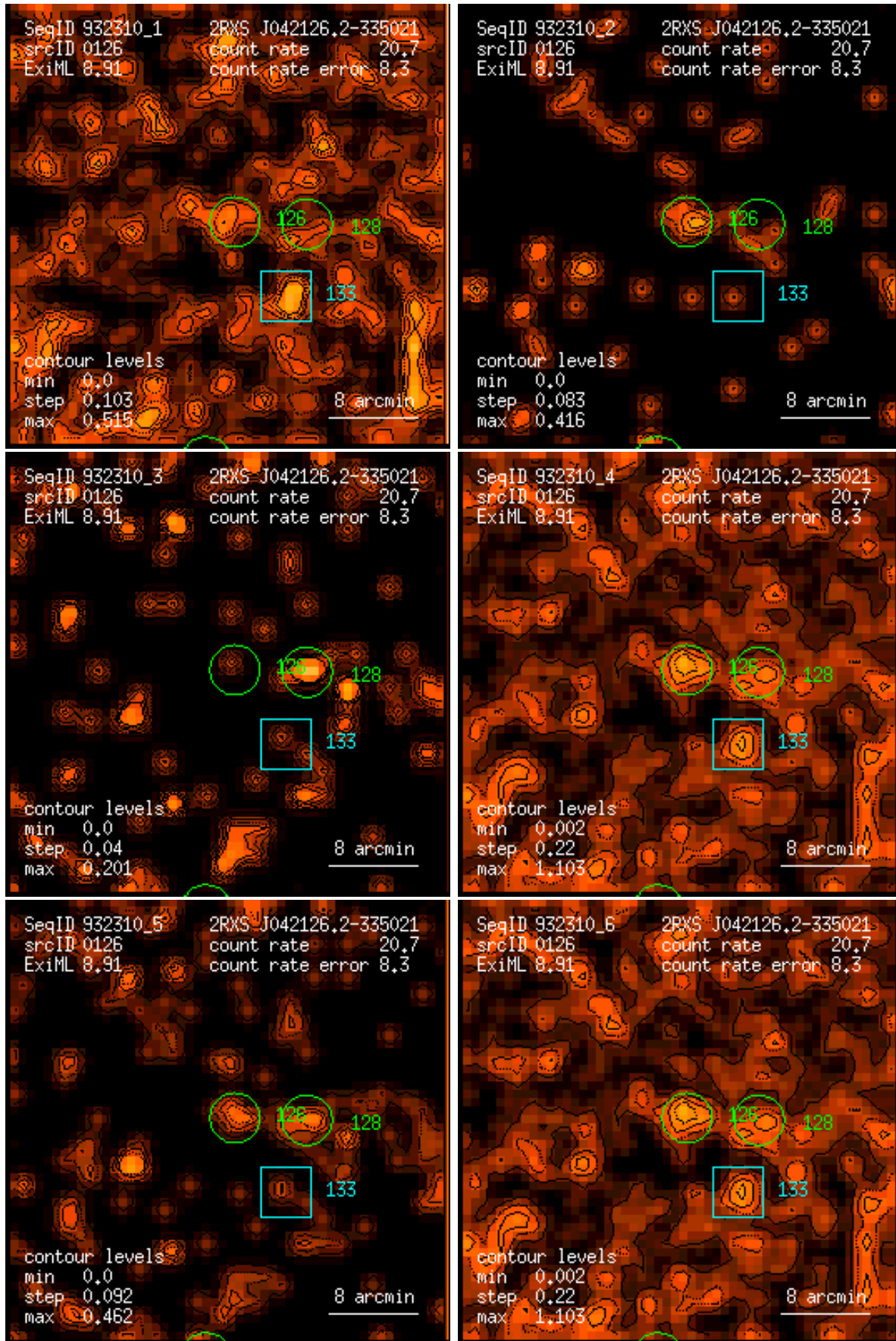
Figure 126: RASS 932310: detection 0126: band rate images, Gaussian filter: (1) PSPC channels 11 – 41, (2) 52 – 90, (3) 91 – 201, (4) 11 – 235, (5) 52 – 201, (6) 11 – 201. Broad band rates in counts/ks. Band rate contour levels in counts/ks/arcmin 2 .
