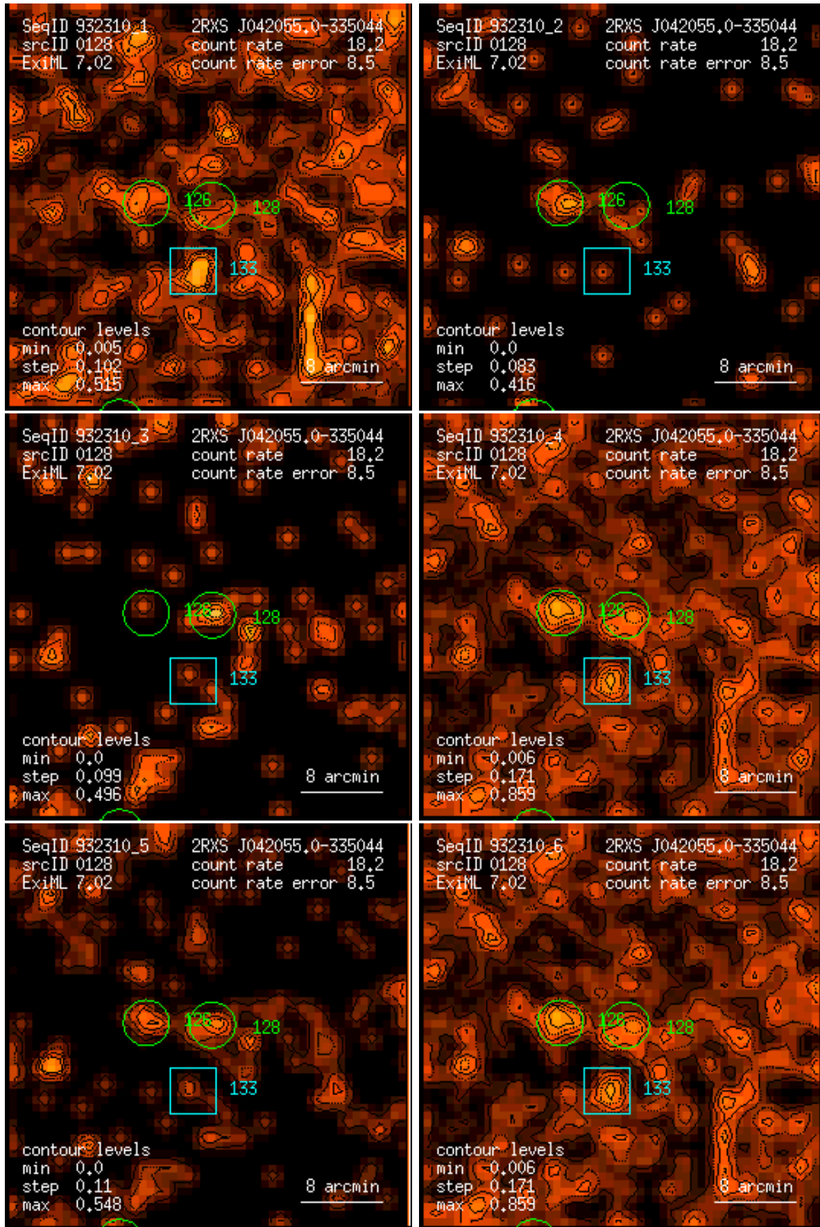
Figure 128: RASS 932310: detection 0128: band rate images, Gaussian filter: (1) PSPC channels 11 – 41, (2) 52 – 90, (3) 91 – 201, (4) 11 – 235, (5) 52 – 201, (6) 11 – 201. Broad band rates in counts/ks. Band rate contour levels in counts/ks/arcmin 2 .
