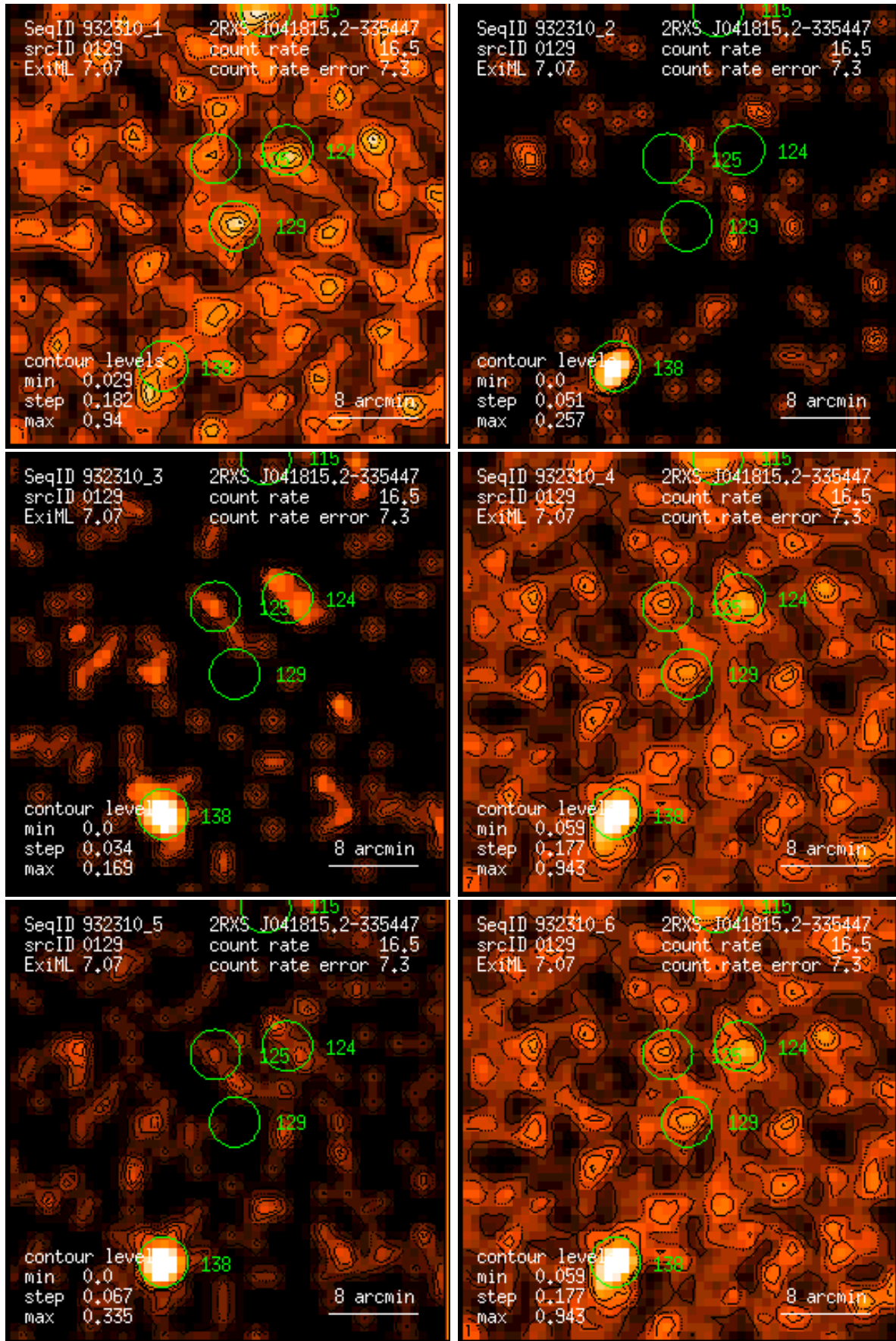
Figure 129: RASS 932310: detection 0129: band rate images, Gaussian filter: (1) PSPC channels 11 – 41, (2) 52 – 90, (3) 91 – 201, (4) 11 – 235, (5) 52 – 201, (6) 11 – 201. Broad band rates in counts/ks. Band rate contour levels in counts/ks/arcmin 2 .
