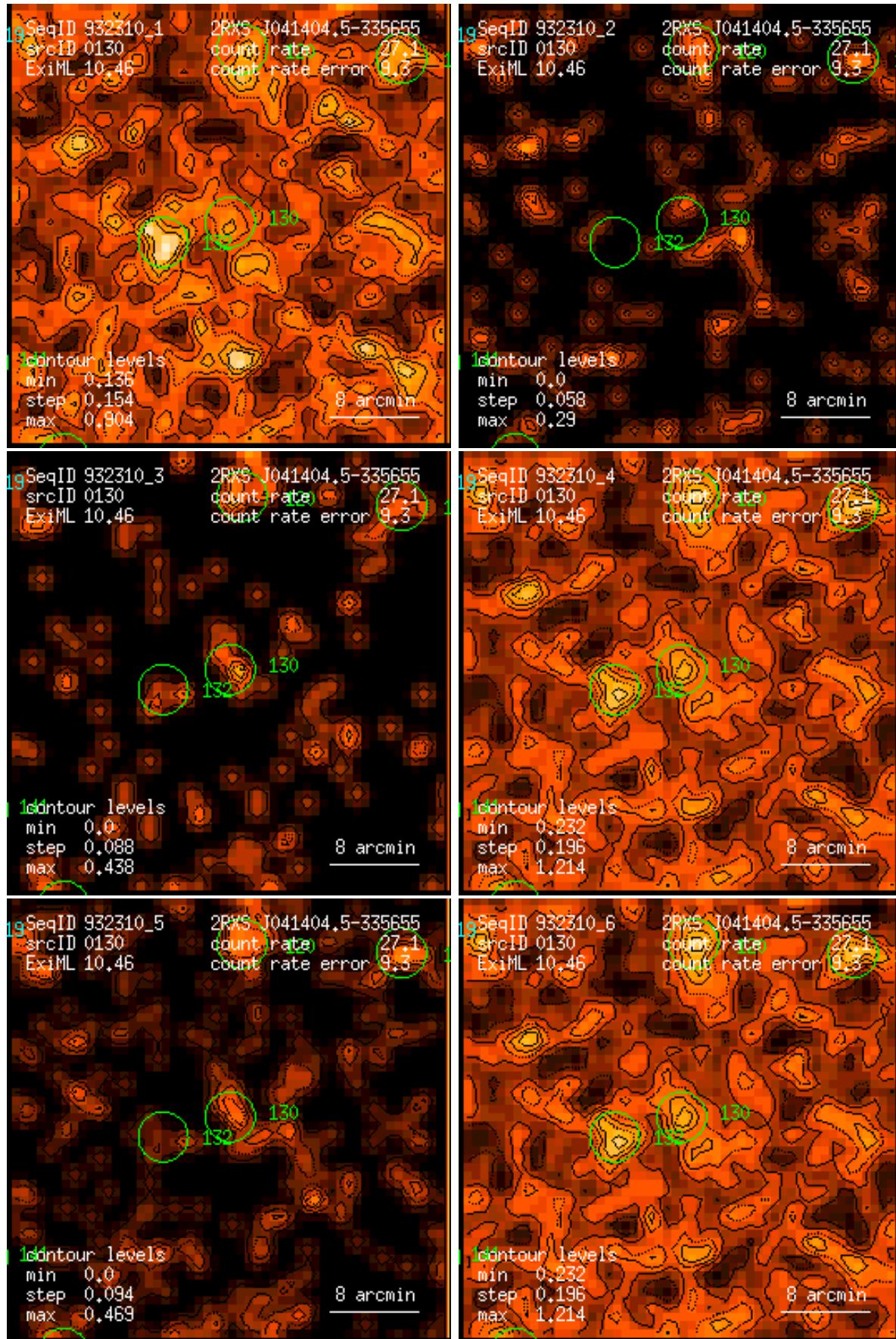
Figure 130: RASS 932310: detection 0130: band rate images, Gaussian filter: (1) PSPC channels 11 – 41, (2) 52 – 90, (3) 91 – 201, (4) 11 – 235, (5) 52 – 201, (6) 11 – 201. Broad band rates in counts/ks. Band rate contour levels in counts/ks/arcmin 2 .
