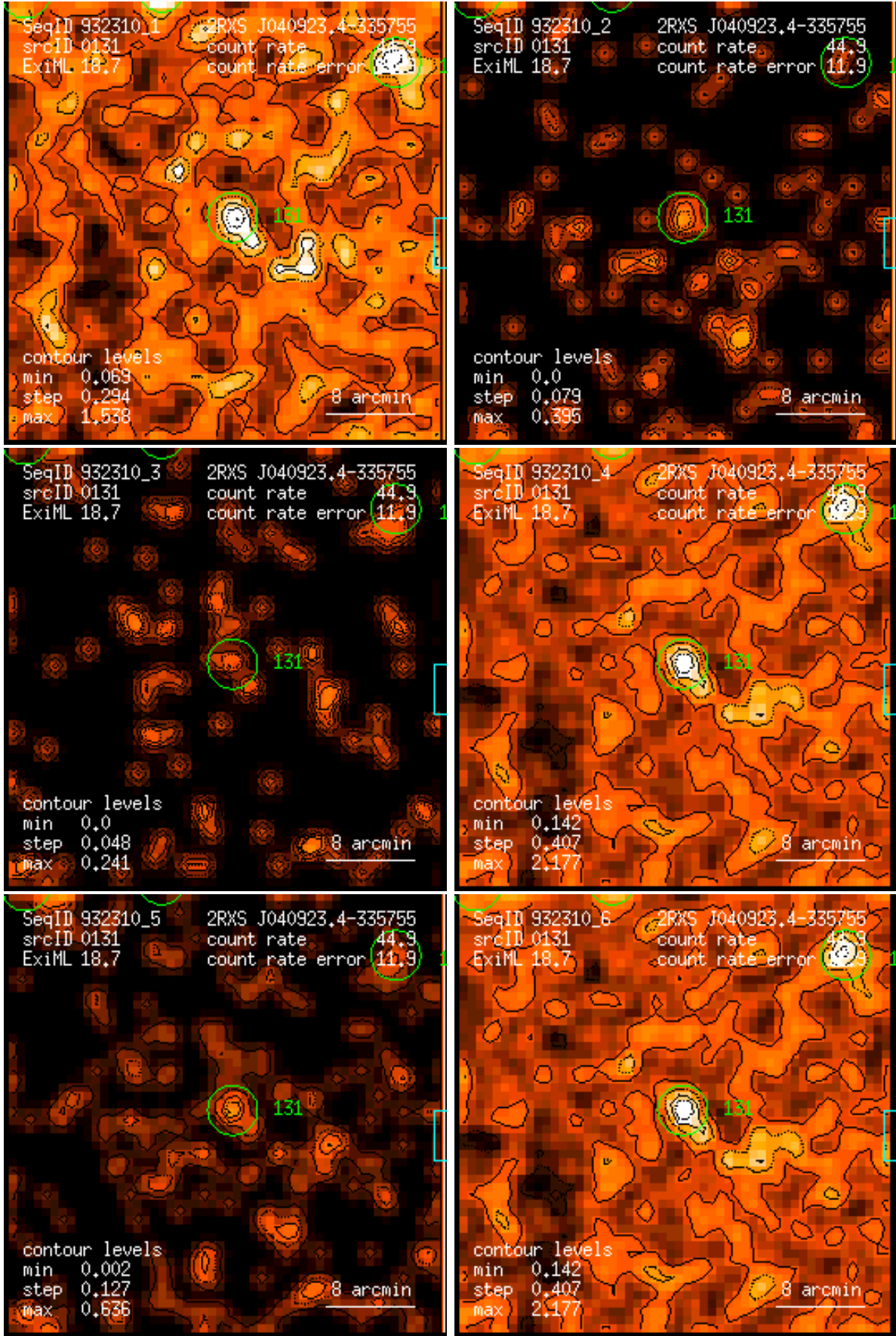
Figure 131: RASS 932310: detection 0131: band rate images, Gaussian filter: (1) PSPC channels 11 – 41, (2) 52 – 90, (3) 91 – 201, (4) 11 – 235, (5) 52 – 201, (6) 11 – 201. Broad band rates in counts/ks. Band rate contour levels in counts/ks/arcmin 2 .
