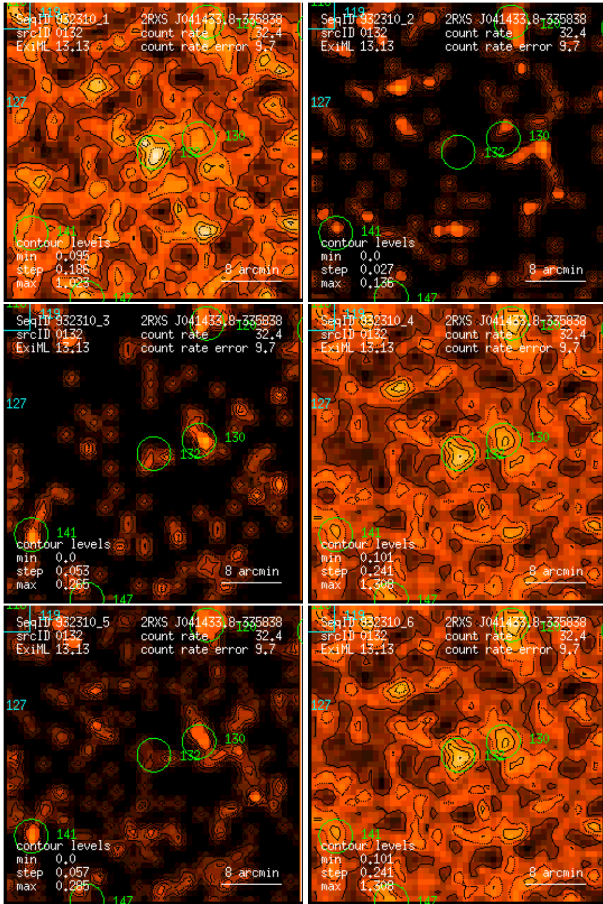
Figure 132: RASS 932310: detection 0132: band rate images, Gaussian filter: (1) PSPC channels 11 – 41, (2) 52 – 90, (3) 91 – 201, (4) 11 – 235, (5) 52 – 201, (6) 11 – 201. Broad band rates in counts/ks. Band rate contour levels in counts/ks/arcmin 2 .
