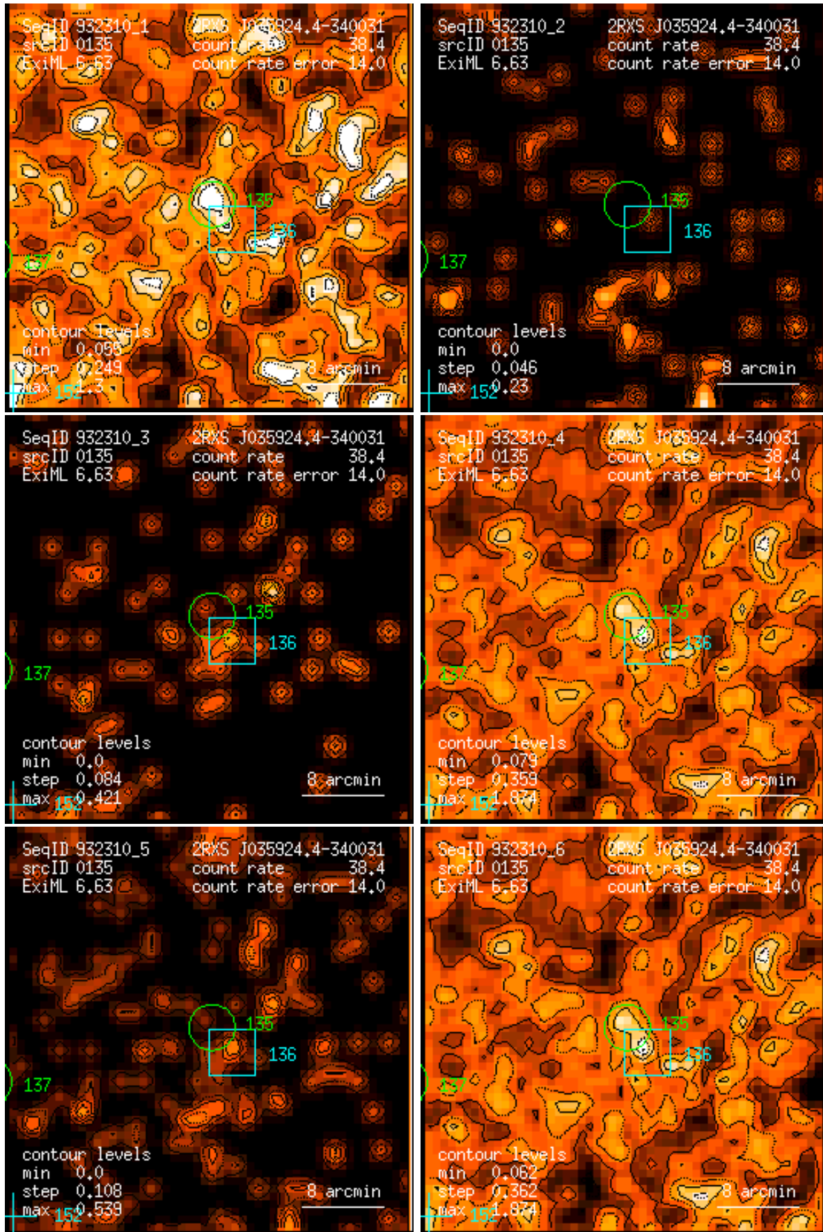
Figure 135: RASS 932310: detection 0135: band rate images, Gaussian filter: (1) PSPC channels 11 – 41, (2) 52 – 90, (3) 91 – 201, (4) 11 – 235, (5) 52 – 201, (6) 11 – 201. Broad band rates in counts/ks. Band rate contour levels in counts/ks/arcmin 2 .
