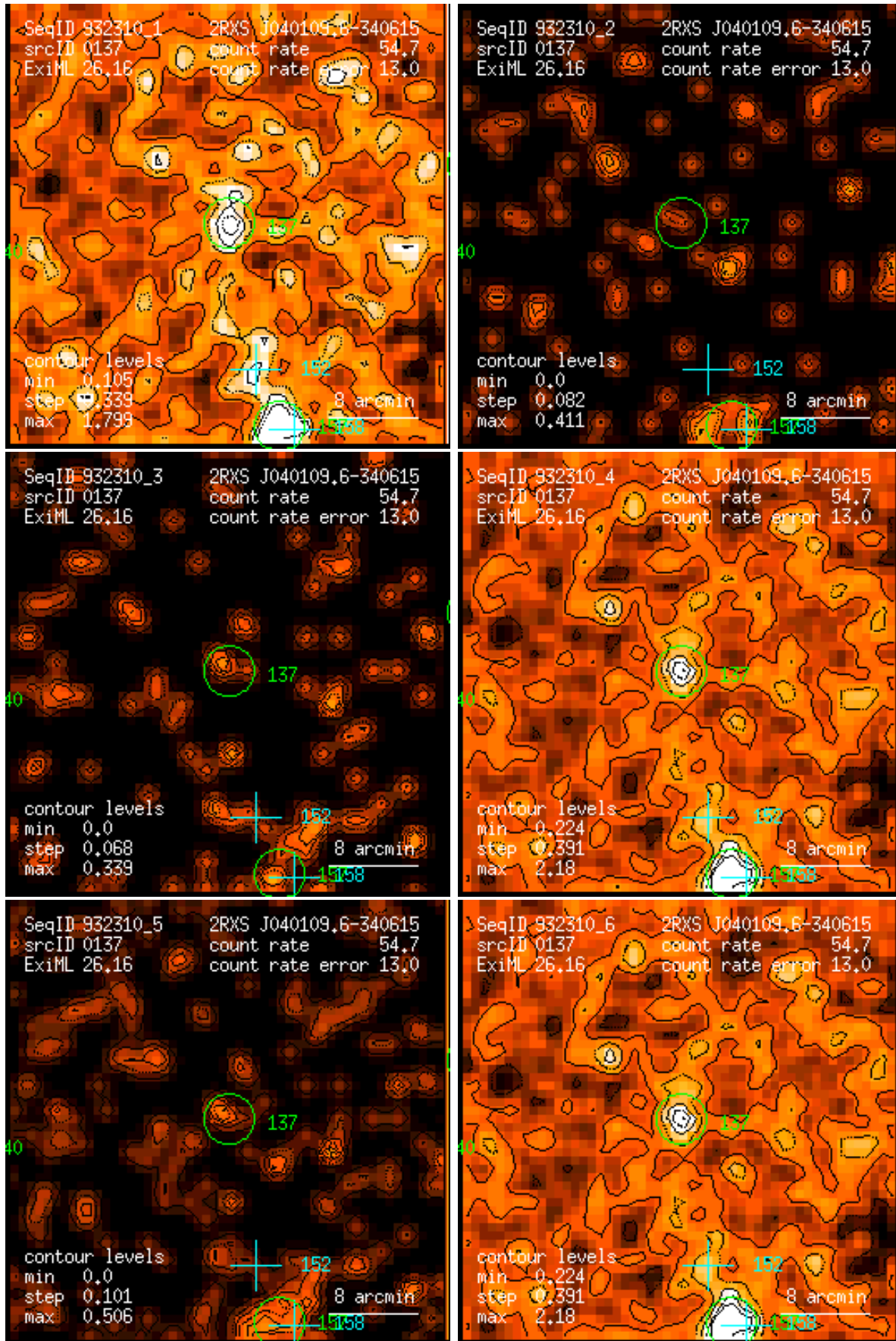
Figure 137: RASS 932310: detection 0137: band rate images, Gaussian filter: (1) PSPC channels 11 – 41, (2) 52 – 90, (3) 91 – 201, (4) 11 – 235, (5) 52 – 201, (6) 11 – 201. Broad band rates in counts/ks. Band rate contour levels in counts/ks/arcmin 2 .
