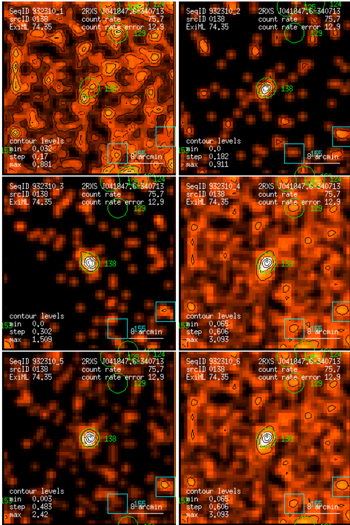
Figure 138: RASS 932310: detection 0138: band rate images, Gaussian filter: (1) PSPC channels 11 – 41, (2) 52 – 90, (3) 91 – 201, (4) 11 – 235, (5) 52 – 201, (6) 11 – 201. Broad band rates in counts/ks. Band rate contour levels in counts/ks/arcmin 2 .
